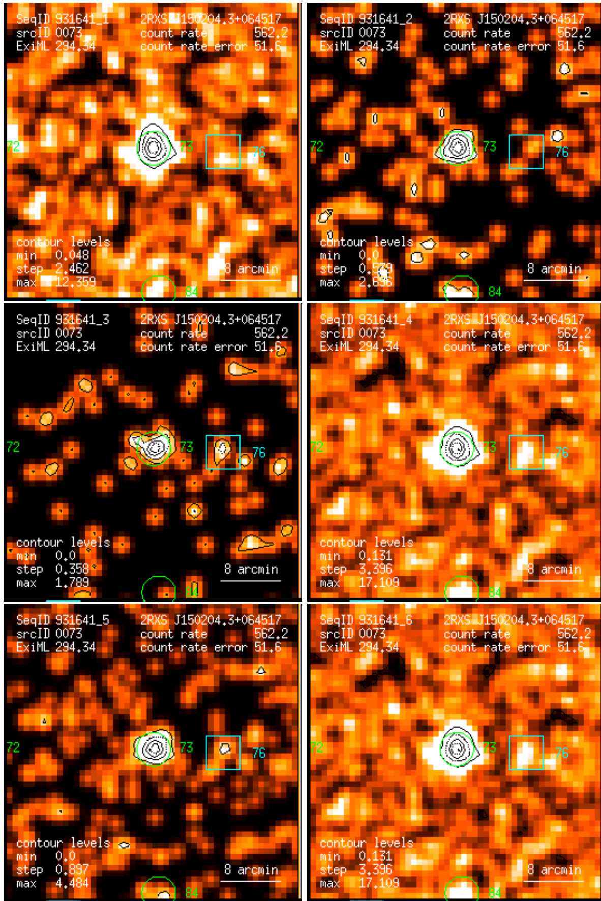
Figure 73: RASS 931641: detection 0073: band rate images, Gaussian filter: (1) PSPC channels 11 – 41, (2) 52 – 90, (3) 91 – 201, (4) 11 – 235, (5) 52 – 201, (6) 11 – 201. Broad band rates in counts/ks. Band rate contour levels in counts/ks/arcmin 2 .
