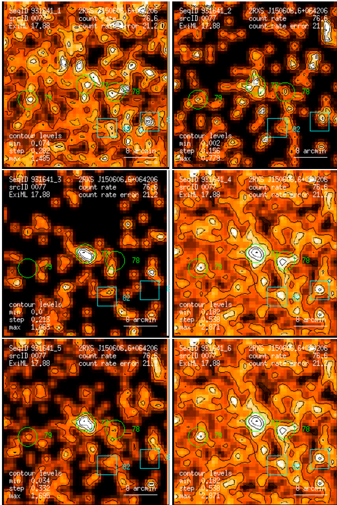
Figure 77: RASS 931641: detection 0077: band rate images, Gaussian filter: (1) PSPC channels 11 – 41, (2) 52 – 90, (3) 91 – 201, (4) 11 – 235, (5) 52 – 201, (6) 11 – 201. Broad band rates in counts/ks. Band rate contour levels in counts/ks/arcmin 2 .
