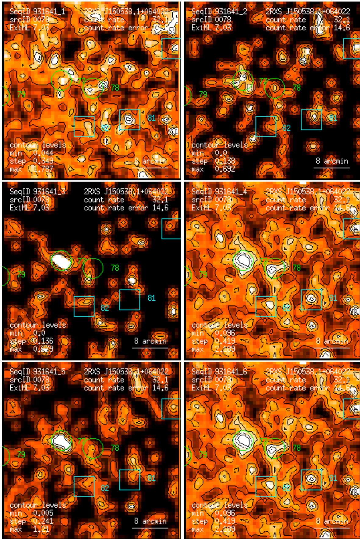
Figure 78: RASS 931641: detection 0078: band rate images, Gaussian filter: (1) PSPC channels 11 – 41, (2) 52 – 90, (3) 91 – 201, (4) 11 – 235, (5) 52 – 201, (6) 11 – 201. Broad band rates in counts/ks. Band rate contour levels in counts/ks/arcmin 2 .
