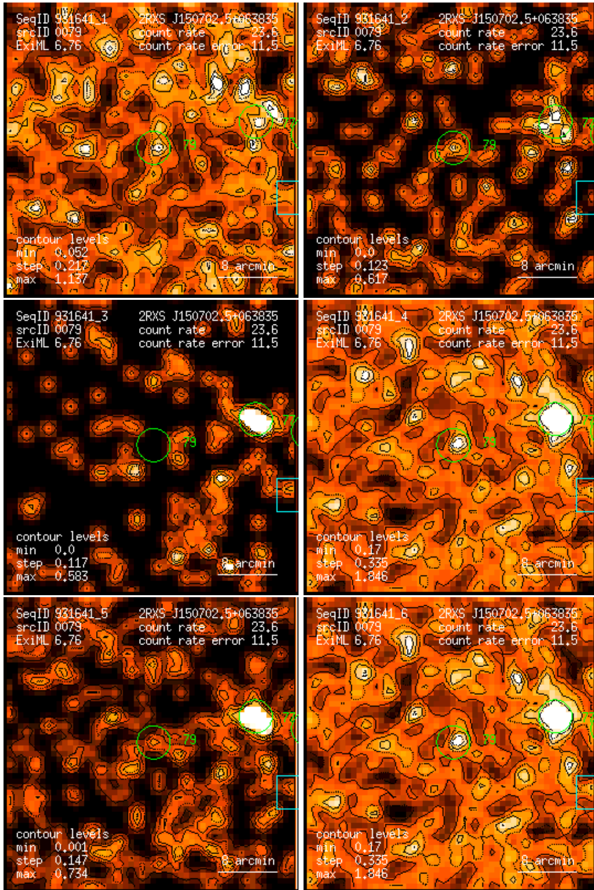
Figure 79: RASS 931641: detection 0079: band rate images, Gaussian filter: (1) PSPC channels 11 – 41, (2) 52 – 90, (3) 91 – 201, (4) 11 – 235, (5) 52 – 201, (6) 11 – 201. Broad band rates in counts/ks. Band rate contour levels in counts/ks/arcmin 2 .
