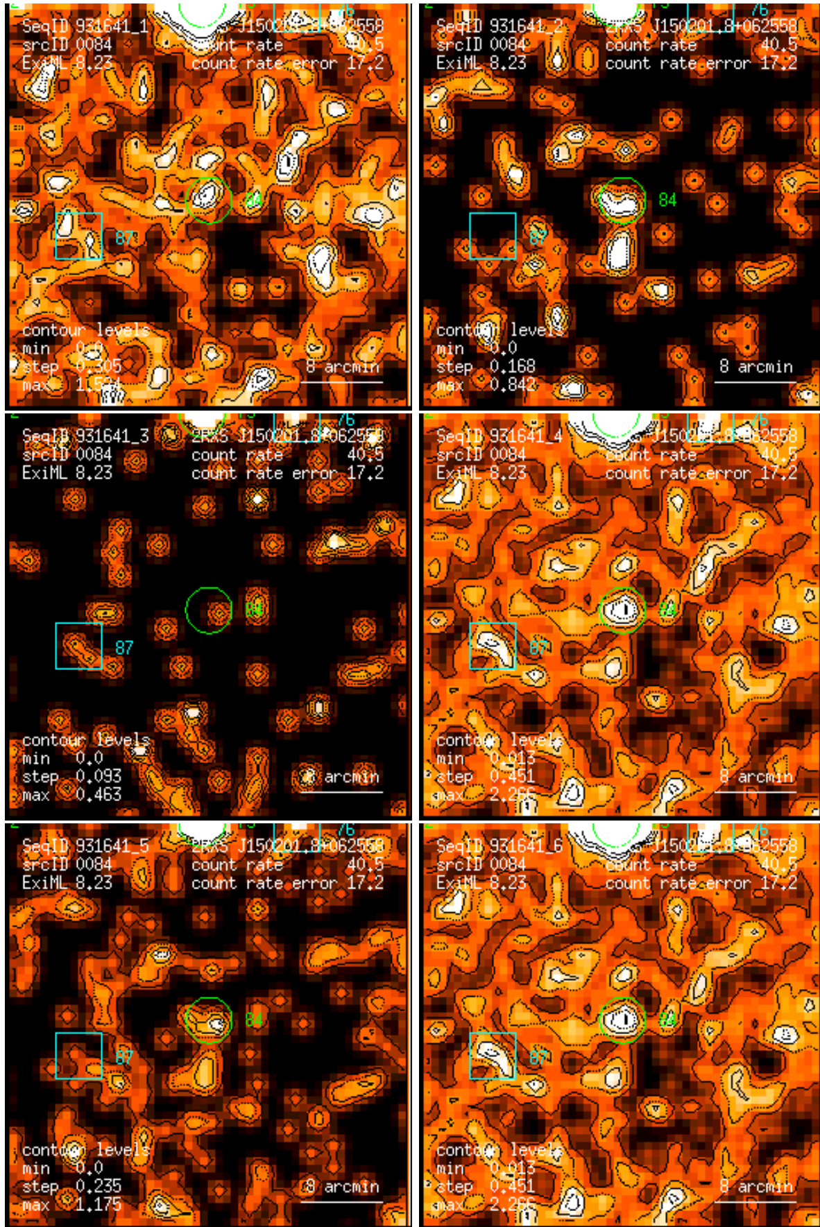
Figure 84: RASS 931641: detection 0084: band rate images, Gaussian filter: (1) PSPC channels 11 – 41, (2) 52 – 90, (3) 91 – 201, (4) 11 – 235, (5) 52 – 201, (6) 11 – 201. Broad band rates in counts/ks. Band rate contour levels in counts/ks/arcmin 2 .
