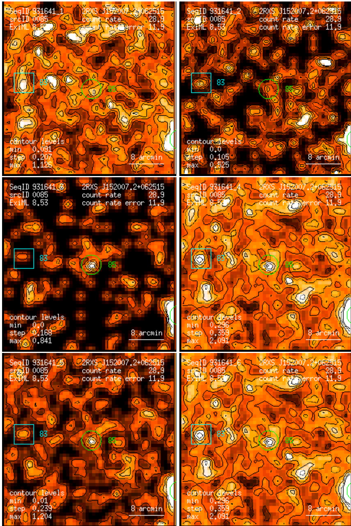
Figure 85: RASS 931641: detection 0085: band rate images, Gaussian filter: (1) PSPC channels 11 – 41, (2) 52 – 90, (3) 91 – 201, (4) 11 – 235, (5) 52 – 201, (6) 11 – 201. Broad band rates in counts/ks. Band rate contour levels in counts/ks/arcmin 2 .
