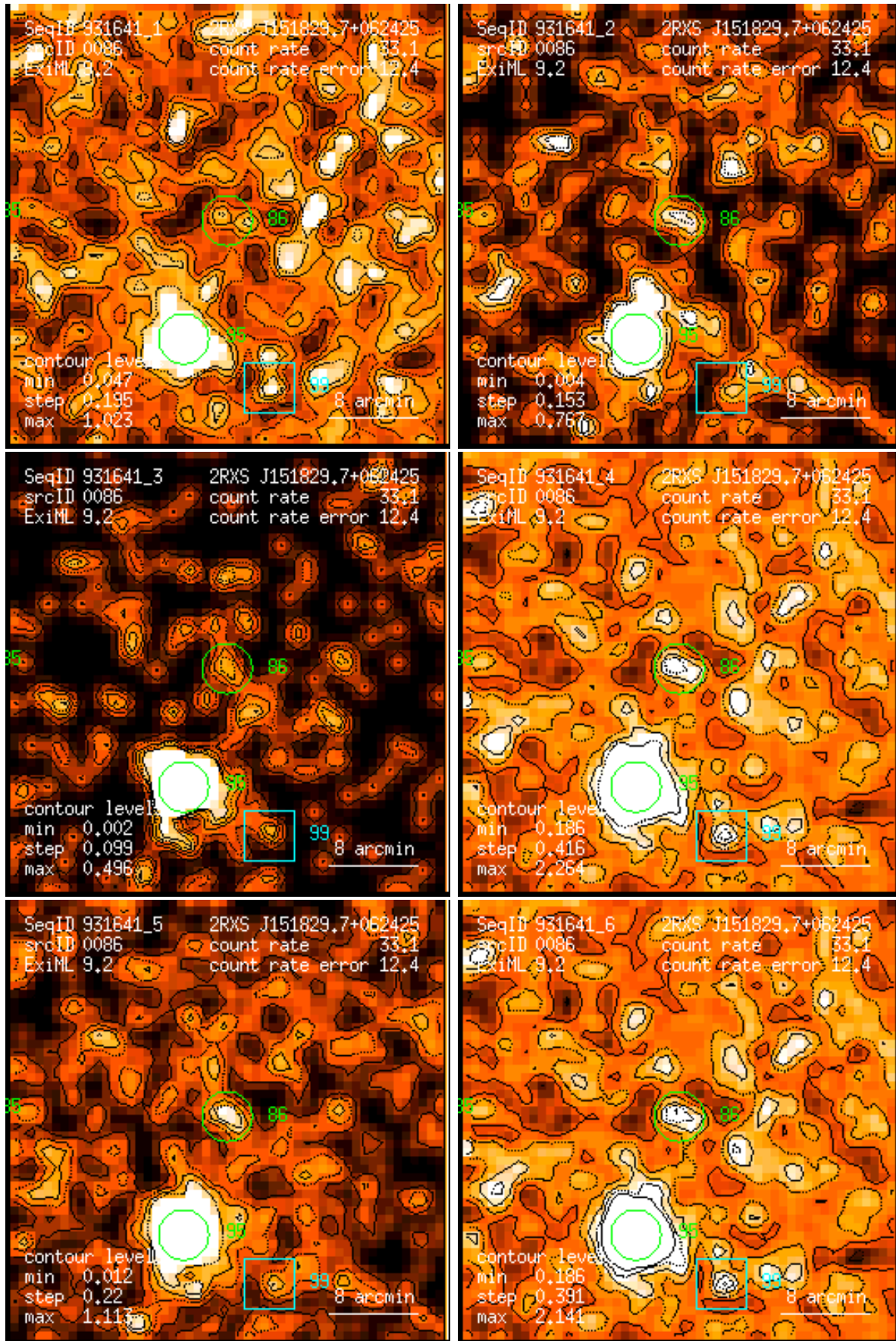
Figure 86: RASS 931641: detection 0086: band rate images, Gaussian filter: (1) PSPC channels 11 – 41, (2) 52 – 90, (3) 91 – 201, (4) 11 – 235, (5) 52 – 201, (6) 11 – 201. Broad band rates in counts/ks. Band rate contour levels in counts/ks/arcmin 2 .
