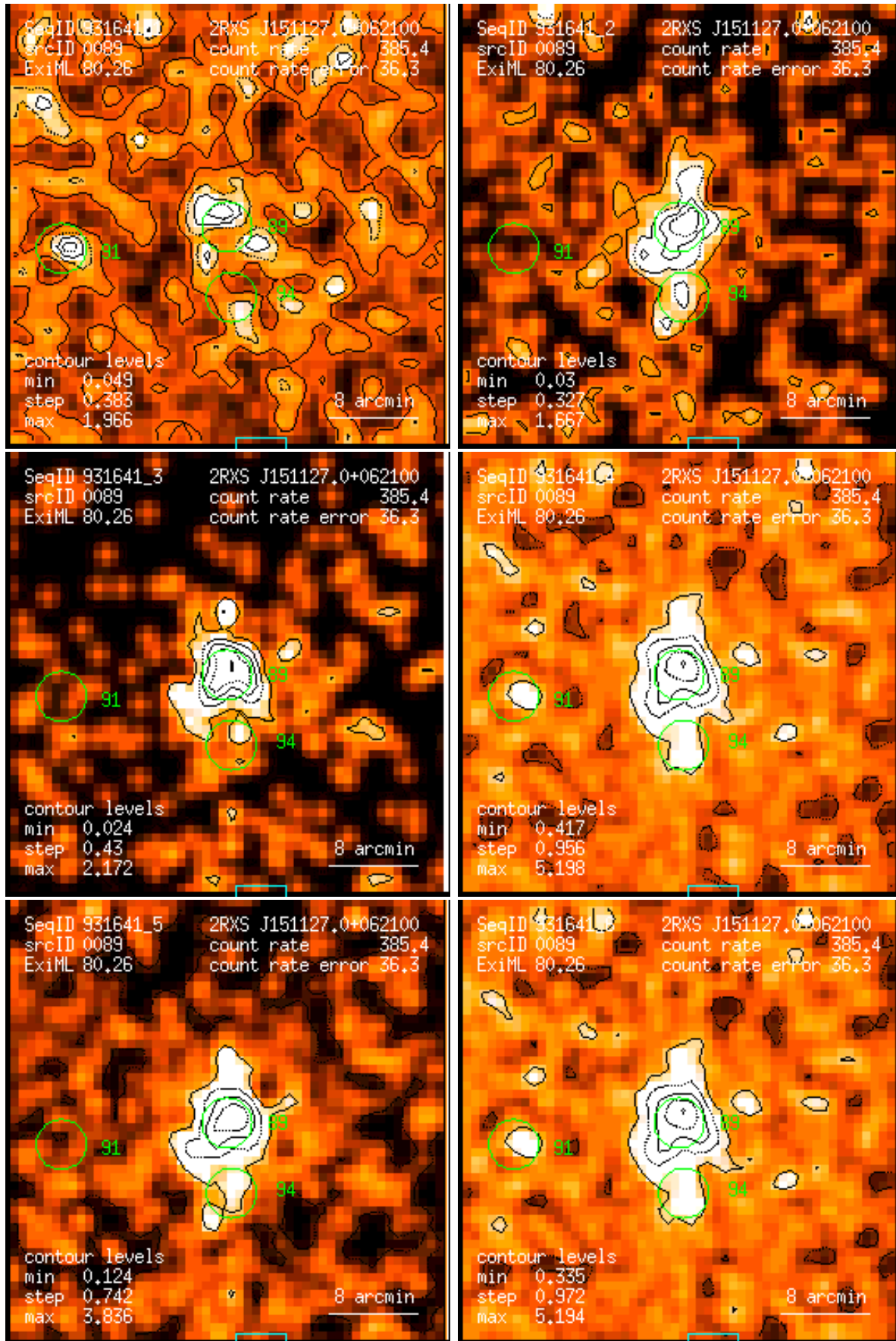
Figure 89: RASS 931641: detection 0089: band rate images, Gaussian filter: (1) PSPC channels 11 – 41, (2) 52 – 90, (3) 91 – 201, (4) 11 – 235, (5) 52 – 201, (6) 11 – 201. Broad band rates in counts/ks. Band rate contour levels in counts/ks/arcmin 2 .
