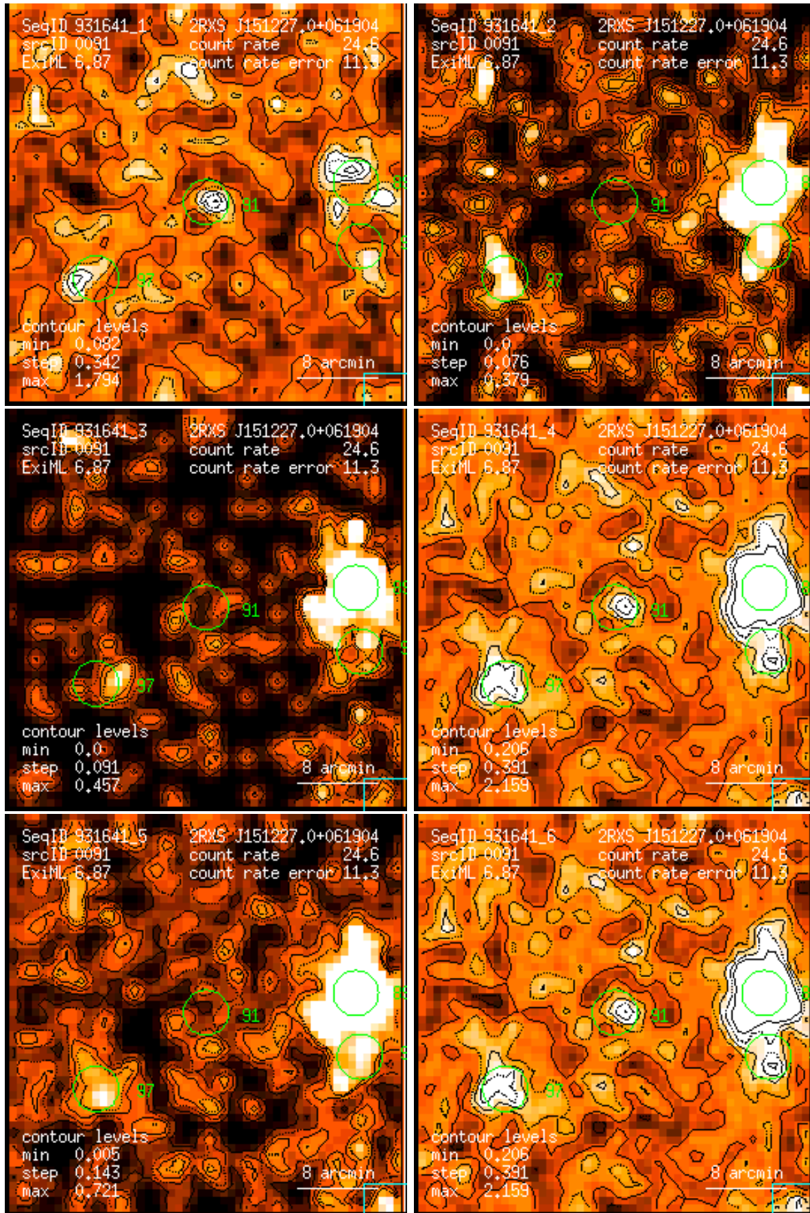
Figure 91: RASS 931641: detection 0091: band rate images, Gaussian filter: (1) PSPC channels 11 – 41, (2) 52 – 90, (3) 91 – 201, (4) 11 – 235, (5) 52 – 201, (6) 11 – 201. Broad band rates in counts/ks. Band rate contour levels in counts/ks/arcmin 2 .
