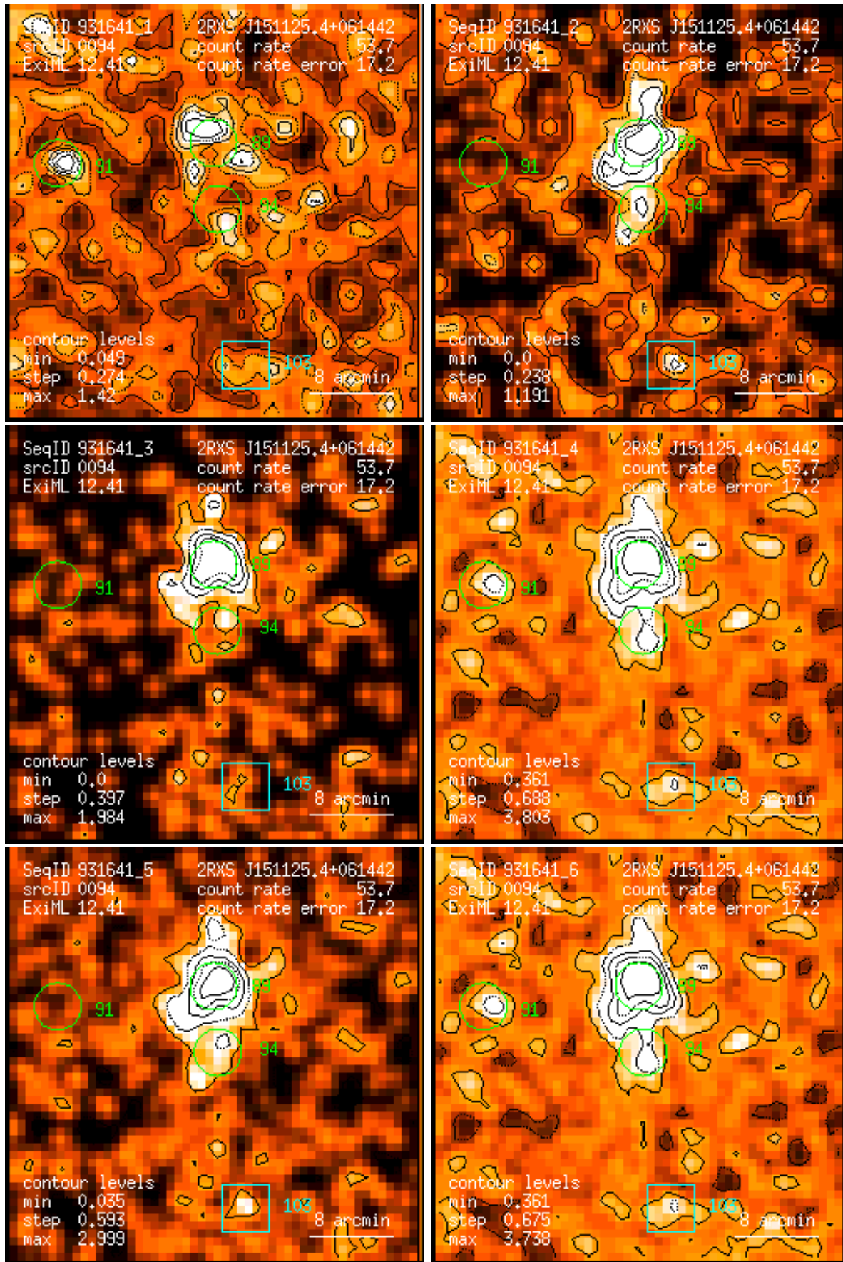
Figure 94: RASS 931641: detection 0094: band rate images, Gaussian filter: (1) PSPC channels 11 – 41, (2) 52 – 90, (3) 91 – 201, (4) 11 – 235, (5) 52 – 201, (6) 11 – 201. Broad band rates in counts/ks. Band rate contour levels in counts/ks/arcmin 2 .
