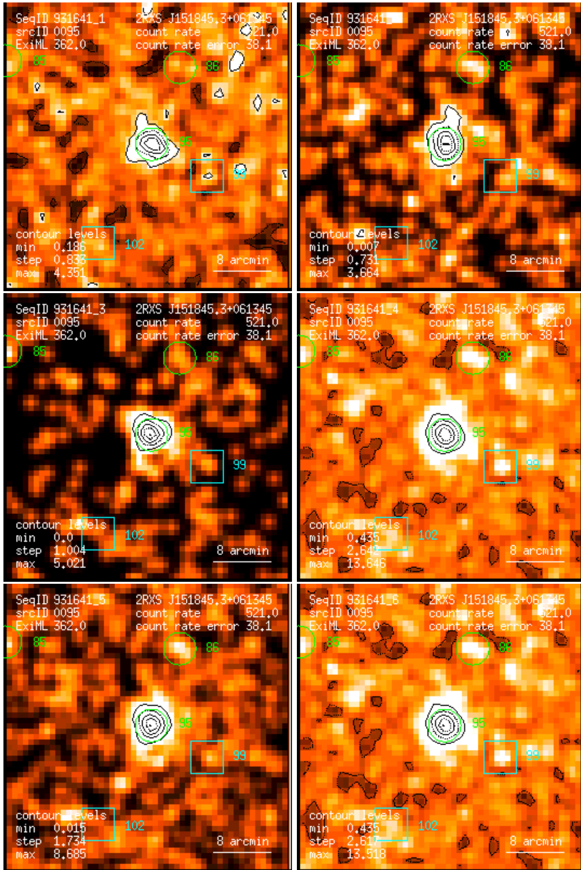
Figure 95: RASS 931641: detection 0095: band rate images, Gaussian filter: (1) PSPC channels 11 – 41, (2) 52 – 90, (3) 91 – 201, (4) 11 – 235, (5) 52 – 201, (6) 11 – 201. Broad band rates in counts/ks. Band rate contour levels in counts/ks/arcmin 2 .
