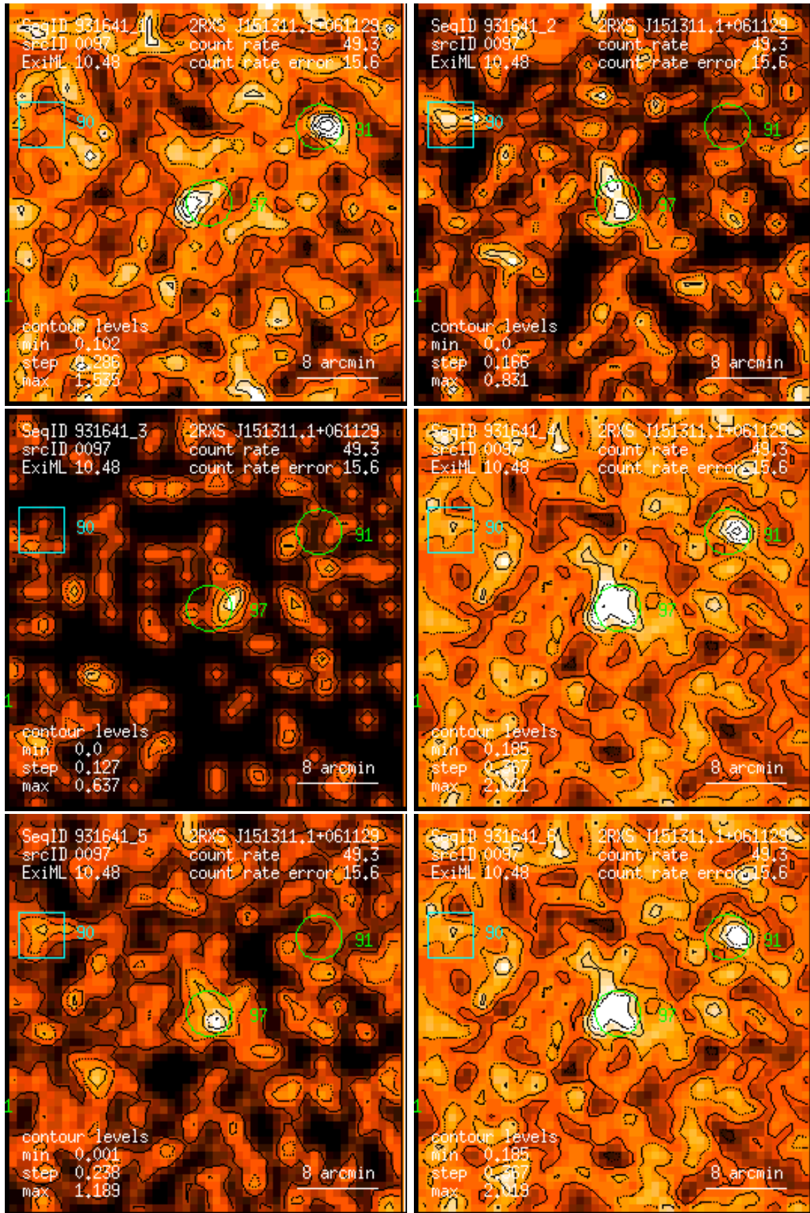
Figure 97: RASS 931641: detection 0097: band rate images, Gaussian filter: (1) PSPC channels 11 – 41, (2) 52 – 90, (3) 91 – 201, (4) 11 – 235, (5) 52 – 201, (6) 11 – 201. Broad band rates in counts/ks. Band rate contour levels in counts/ks/arcmin 2 .
