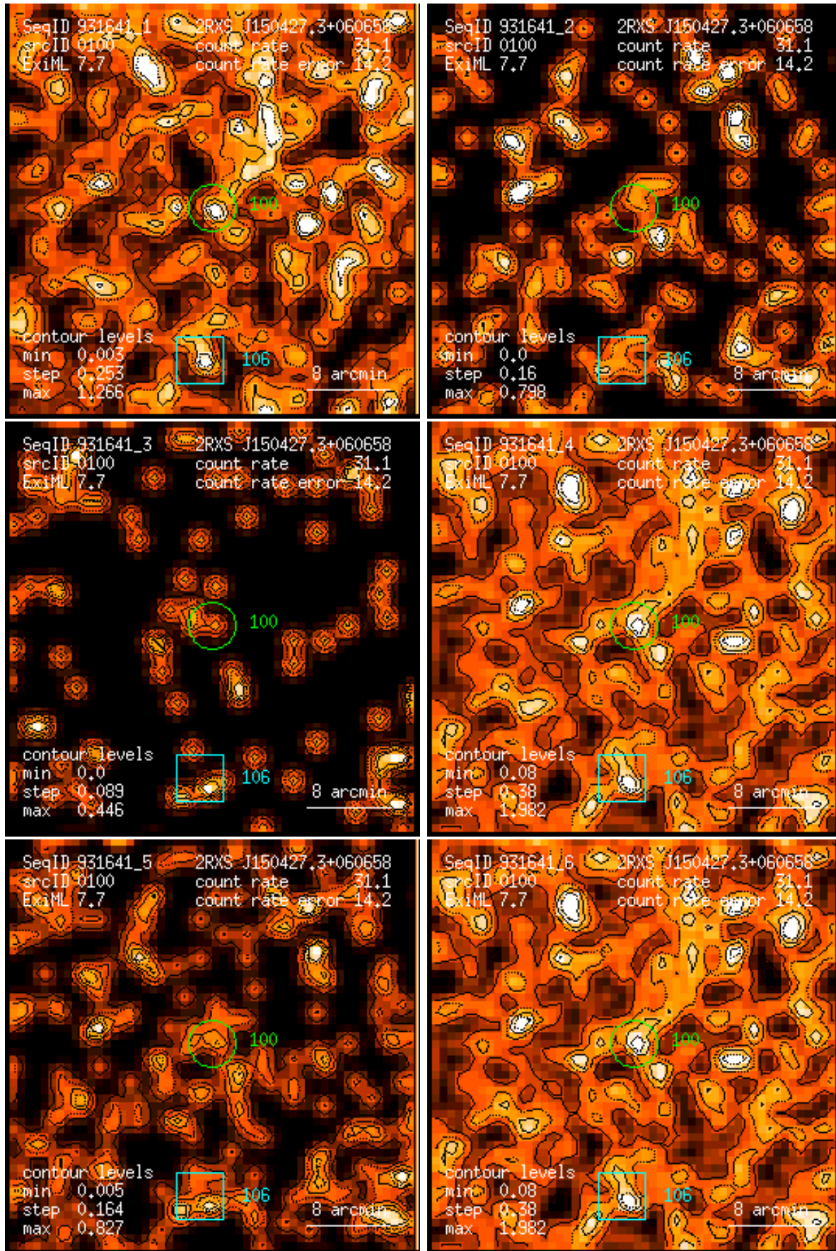
Figure 100: RASS 931641: detection 0100: band rate images, Gaussian filter: (1) PSPC channels 11 – 41, (2) 52 – 90, (3) 91 – 201, (4) 11 – 235, (5) 52 – 201, (6) 11 – 201. Broad band rates in counts/ks. Band rate contour levels in counts/ks/arcmin 2 .
