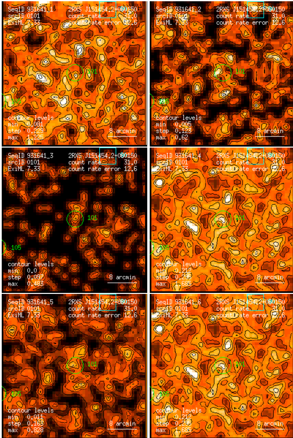
Figure 101: RASS 931641: detection 0101: band rate images, Gaussian filter: (1) PSPC channels 11 – 41, (2) 52 – 90, (3) 91 – 201, (4) 11 – 235, (5) 52 – 201, (6) 11 – 201. Broad band rates in counts/ks. Band rate contour levels in counts/ks/arcmin 2 .
