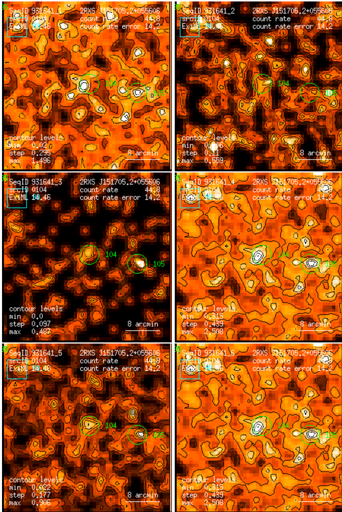
Figure 104: RASS 931641: detection 0104: band rate images, Gaussian filter: (1) PSPC channels 11 – 41, (2) 52 – 90, (3) 91 – 201, (4) 11 – 235, (5) 52 – 201, (6) 11 – 201. Broad band rates in counts/ks. Band rate contour levels in counts/ks/arcmin 2 .
