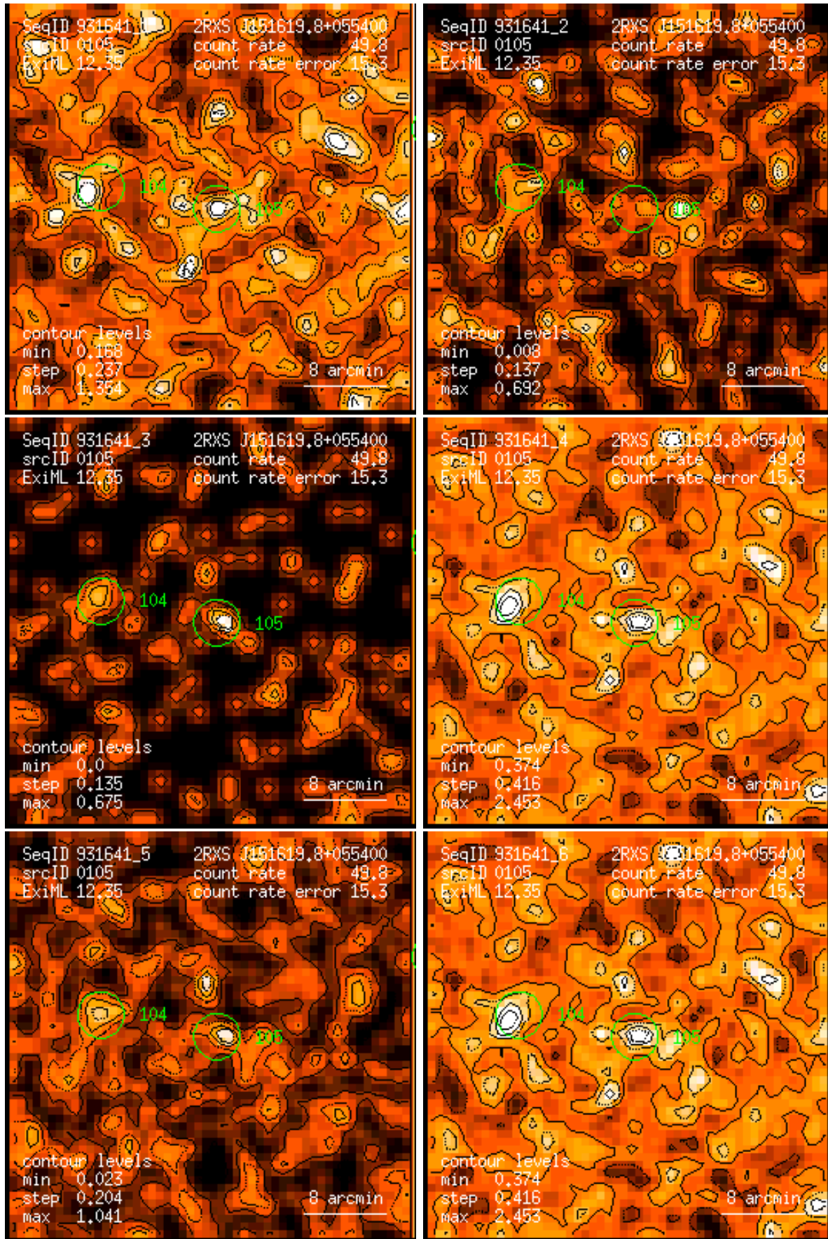
Figure 105: RASS 931641: detection 0105: band rate images, Gaussian filter: (1) PSPC channels 11 – 41, (2) 52 – 90, (3) 91 – 201, (4) 11 – 235, (5) 52 – 201, (6) 11 – 201. Broad band rates in counts/ks. Band rate contour levels in counts/ks/arcmin 2 .
