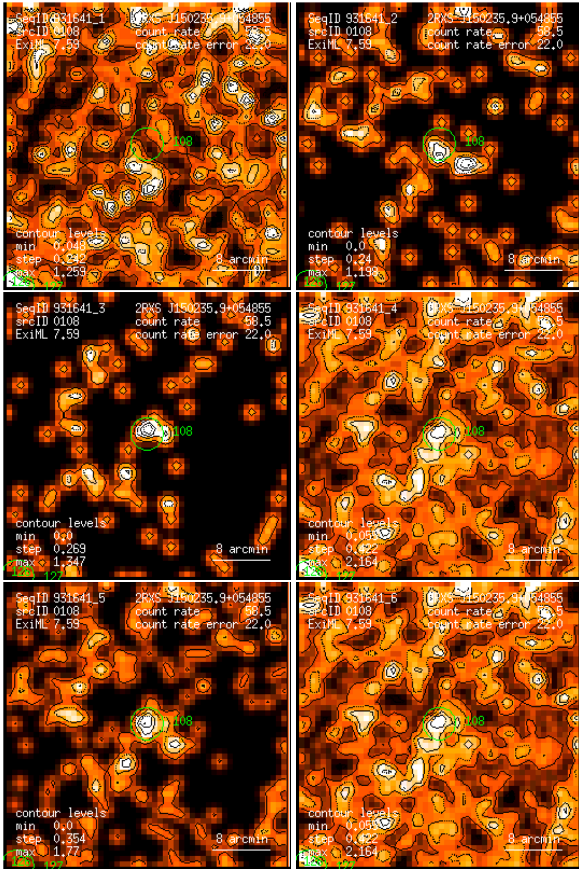
Figure 108: RASS 931641: detection 0108: band rate images, Gaussian filter: (1) PSPC channels 11 – 41, (2) 52 – 90, (3) 91 – 201, (4) 11 – 235, (5) 52 – 201, (6) 11 – 201. Broad band rates in counts/ks. Band rate contour levels in counts/ks/arcmin 2 .
