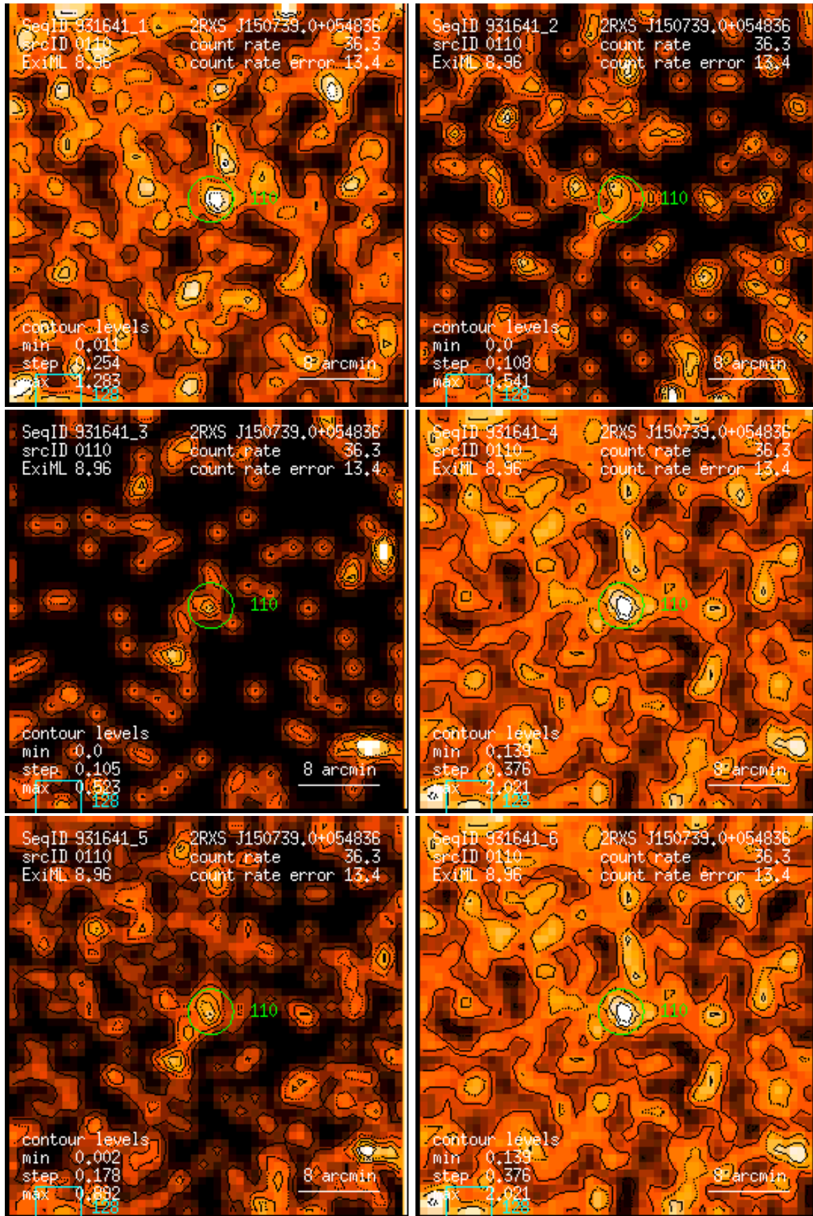
Figure 110: RASS 931641: detection 0110: band rate images, Gaussian filter: (1) PSPC channels 11 – 41, (2) 52 – 90, (3) 91 – 201, (4) 11 – 235, (5) 52 – 201, (6) 11 – 201. Broad band rates in counts/ks. Band rate contour levels in counts/ks/arcmin 2 .
