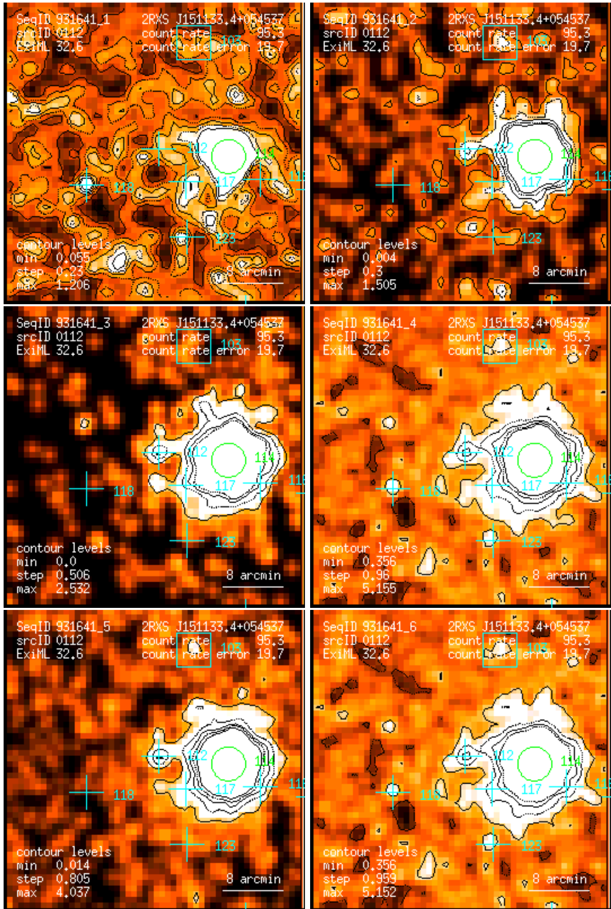
Figure 112: RASS 931641: detection 0112: band rate images, Gaussian filter: (1) PSPC channels 11 – 41, (2) 52 – 90, (3) 91 – 201, (4) 11 – 235, (5) 52 – 201, (6) 11 – 201. Broad band rates in counts/ks. Band rate contour levels in counts/ks/arcmin 2 .
