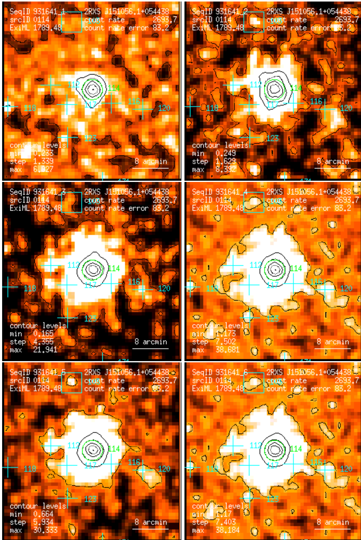
Figure 114: RASS 931641: detection 0114: band rate images, Gaussian filter: (1) PSPC channels 11 – 41, (2) 52 – 90, (3) 91 – 201, (4) 11 – 235, (5) 52 – 201, (6) 11 – 201. Broad band rates in counts/ks. Band rate contour levels in counts/ks/arcmin 2 .
