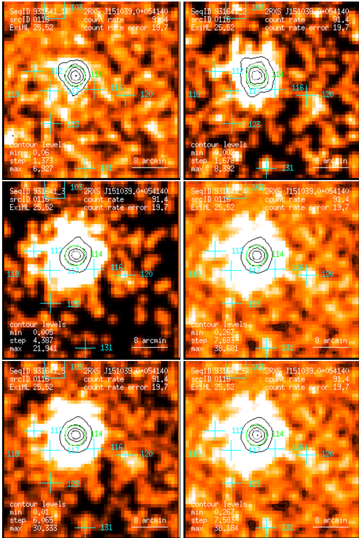
Figure 116: RASS 931641: detection 0116: band rate images, Gaussian filter: (1) PSPC channels 11 – 41, (2) 52 – 90, (3) 91 – 201, (4) 11 – 235, (5) 52 – 201, (6) 11 – 201. Broad band rates in counts/ks. Band rate contour levels in counts/ks/arcmin 2 .
