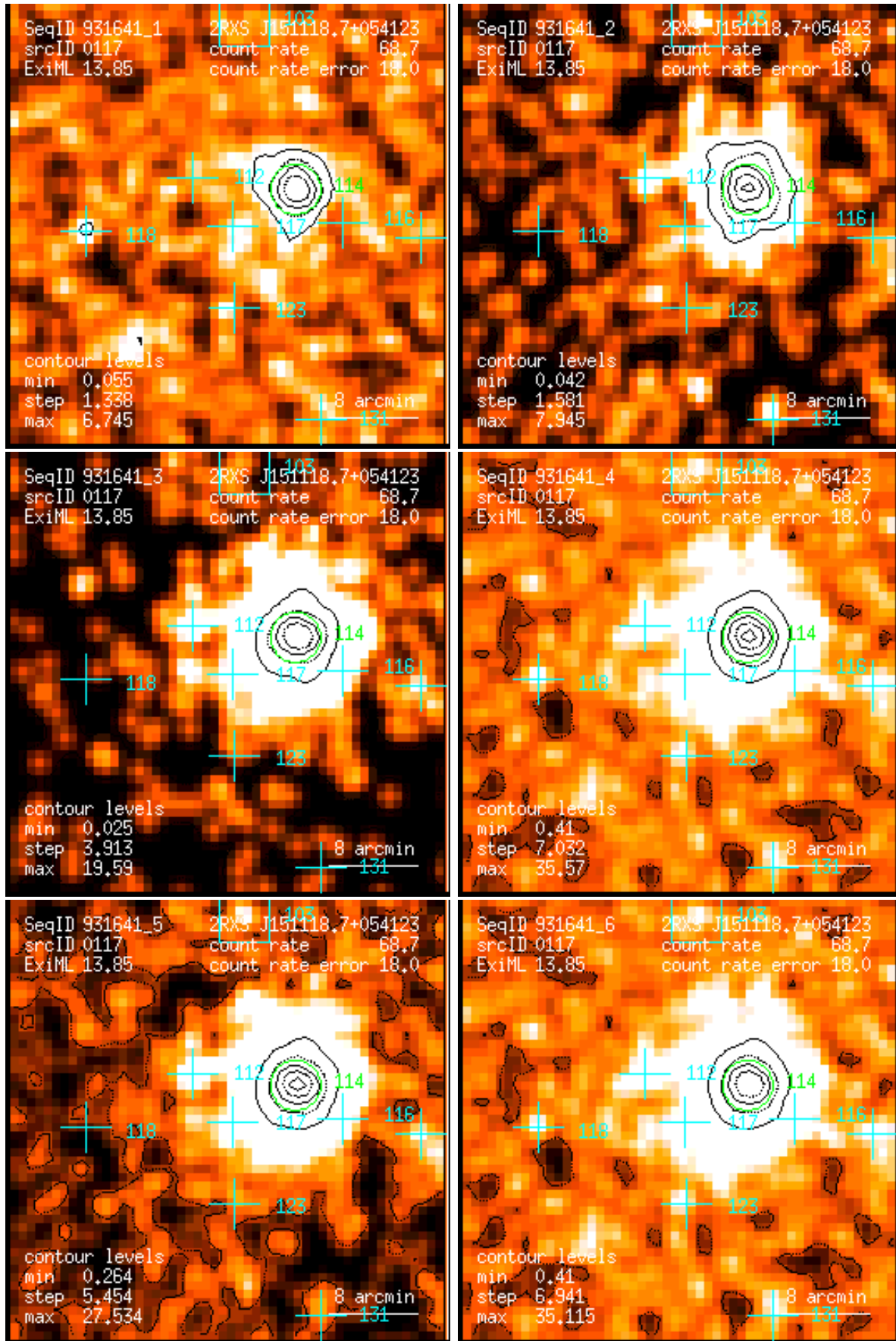
Figure 117: RASS 931641: detection 0117: band rate images, Gaussian filter: (1) PSPC channels 11 – 41, (2) 52 – 90, (3) 91 – 201, (4) 11 – 235, (5) 52 – 201, (6) 11 – 201. Broad band rates in counts/ks. Band rate contour levels in counts/ks/arcmin 2 .
