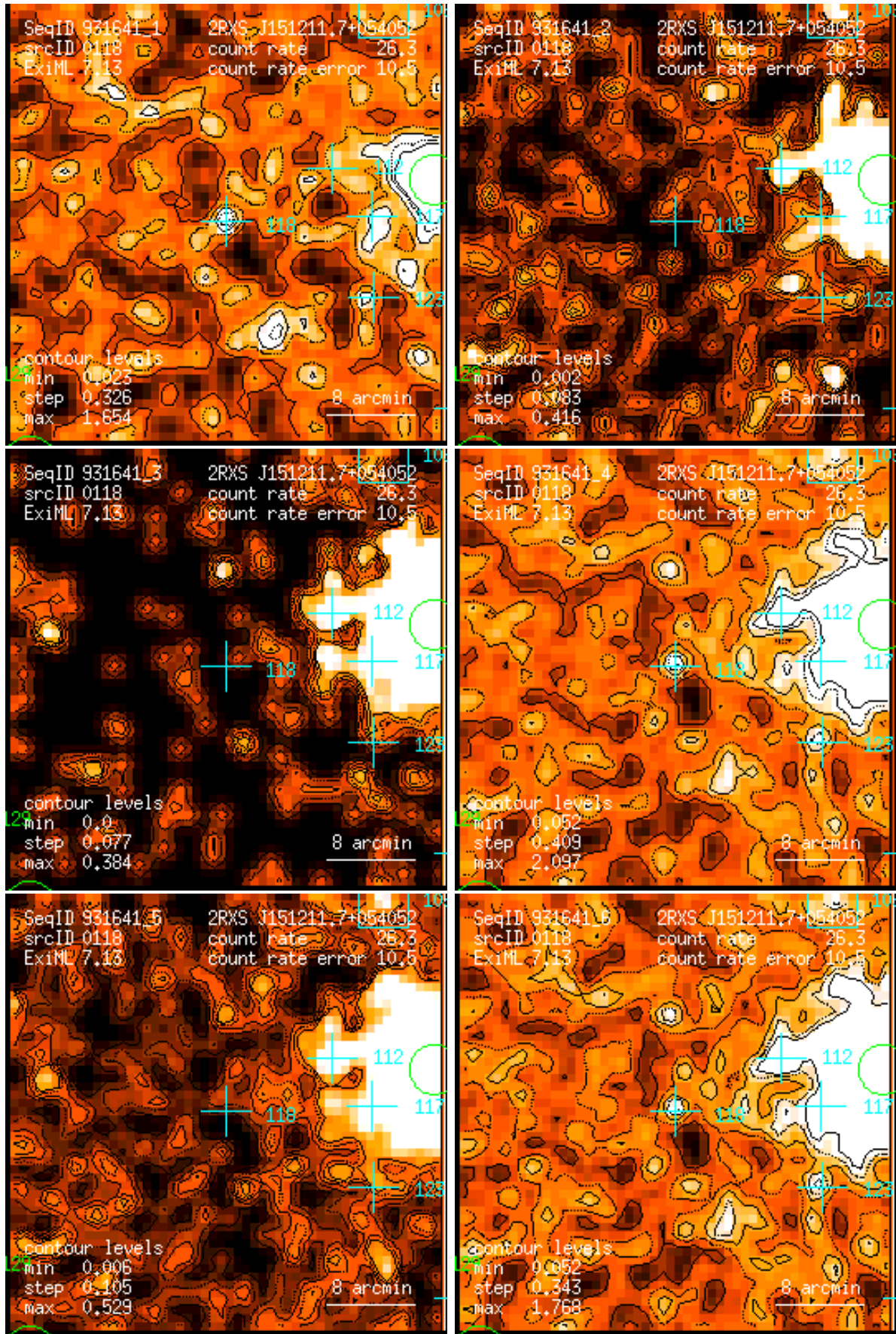
Figure 118: RASS 931641: detection 0118: band rate images, Gaussian filter: (1) PSPC channels 11 – 41, (2) 52 – 90, (3) 91 – 201, (4) 11 – 235, (5) 52 – 201, (6) 11 – 201. Broad band rates in counts/ks. Band rate contour levels in counts/ks/arcmin 2 .
