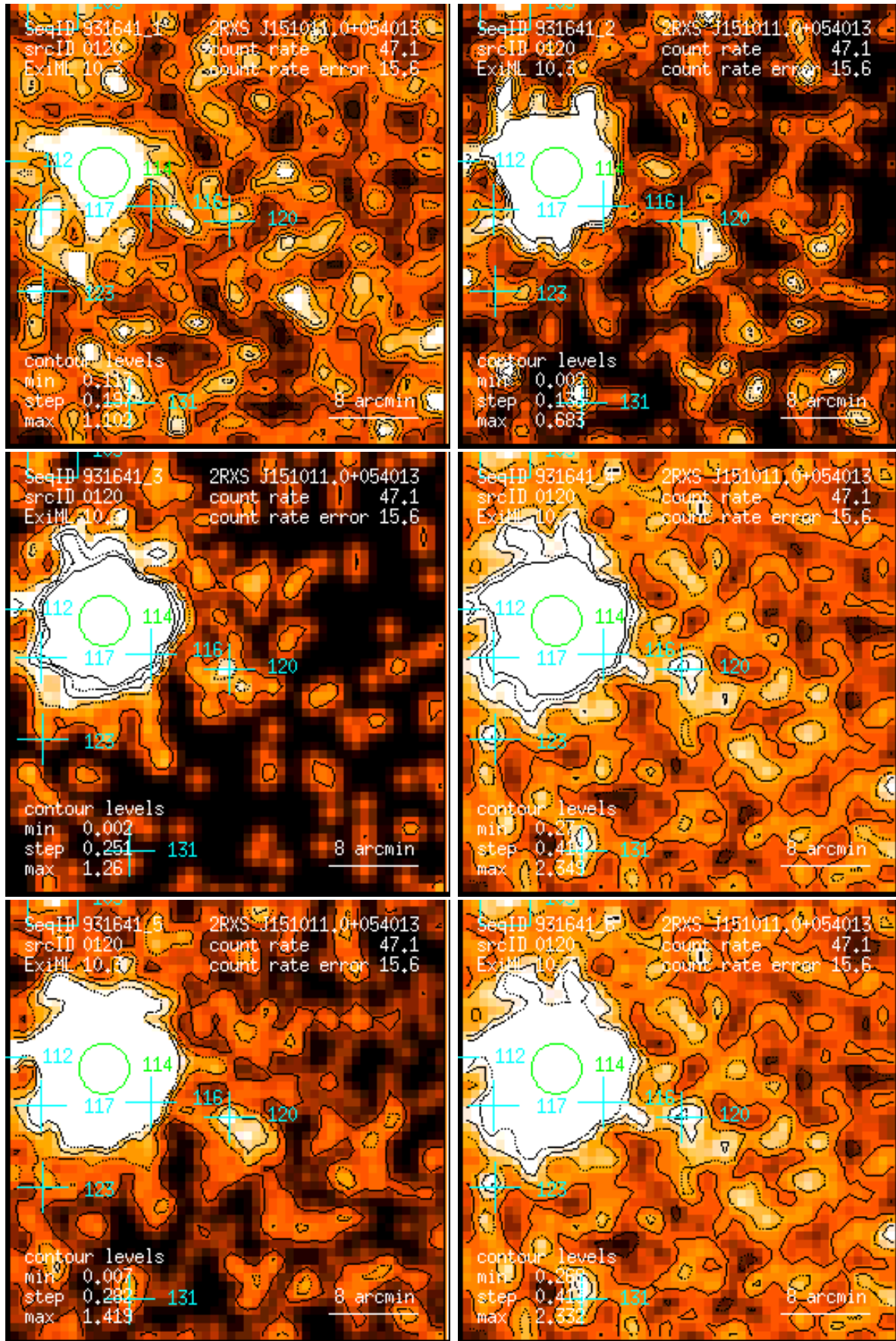
Figure 120: RASS 931641: detection 0120: band rate images, Gaussian filter: (1) PSPC channels 11 – 41, (2) 52 – 90, (3) 91 – 201, (4) 11 – 235, (5) 52 – 201, (6) 11 – 201. Broad band rates in counts/ks. Band rate contour levels in counts/ks/arcmin 2 .
