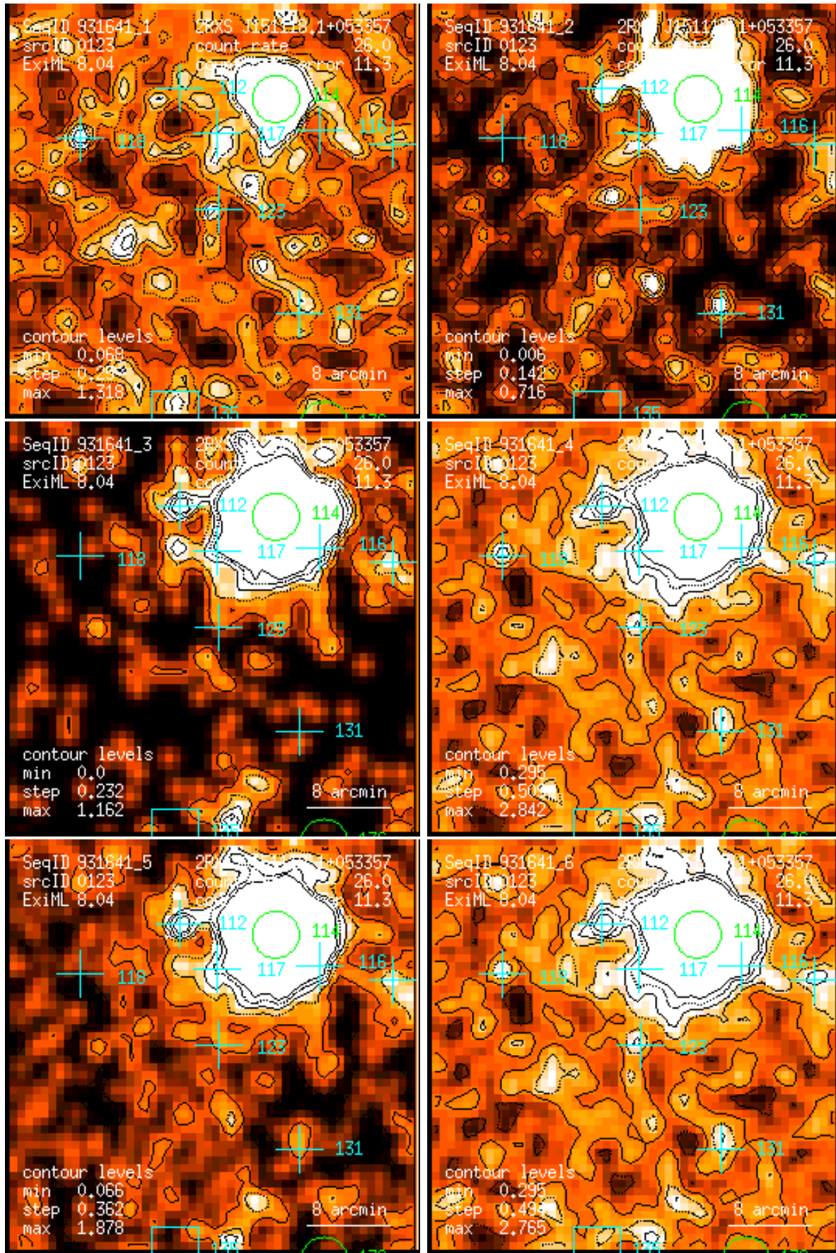
Figure 123: RASS 931641: detection 0123: band rate images, Gaussian filter: (1) PSPC channels 11 – 41, (2) 52 – 90, (3) 91 – 201, (4) 11 – 235, (5) 52 – 201, (6) 11 – 201. Broad band rates in counts/ks. Band rate contour levels in counts/ks/arcmin 2 .
