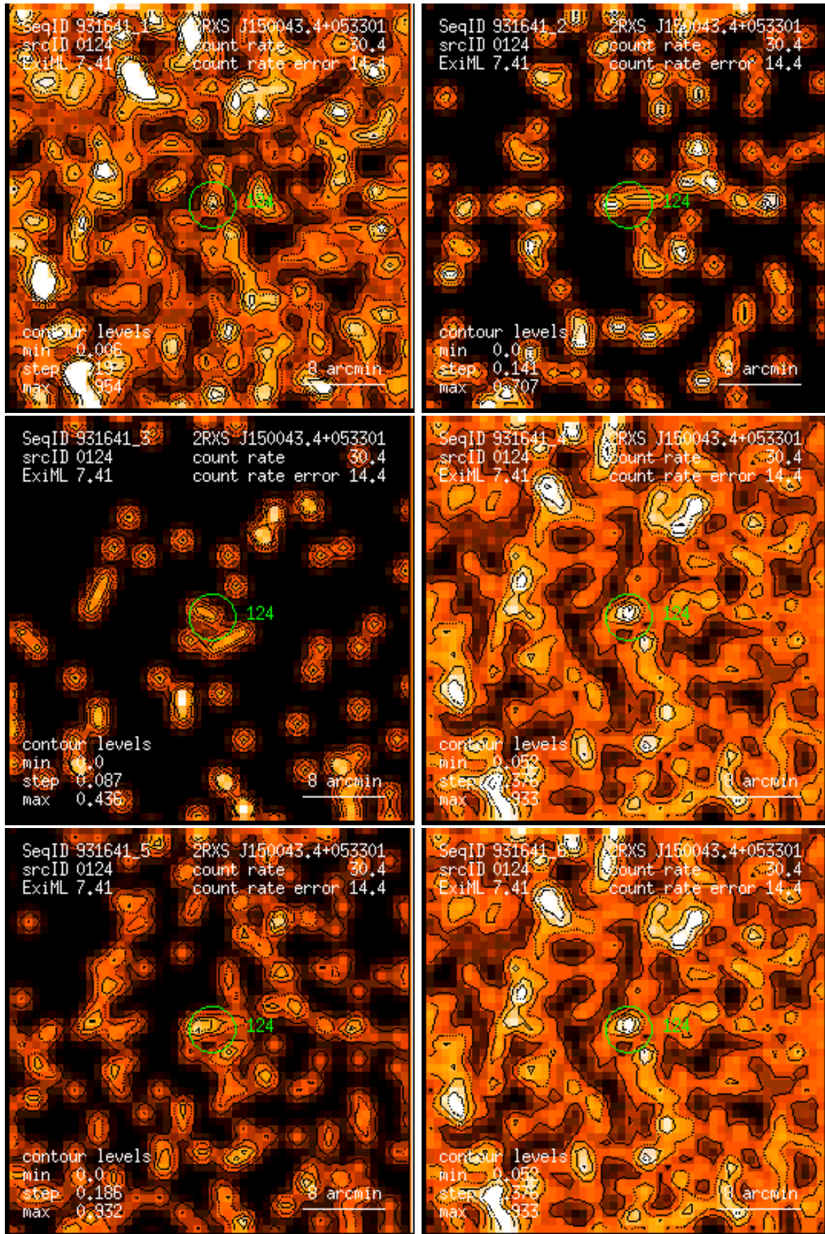
Figure 124: RASS 931641: detection 0124: band rate images, Gaussian filter: (1) PSPC channels 11 – 41, (2) 52 – 90, (3) 91 – 201, (4) 11 – 235, (5) 52 – 201, (6) 11 – 201. Broad band rates in counts/ks. Band rate contour levels in counts/ks/arcmin 2 .
