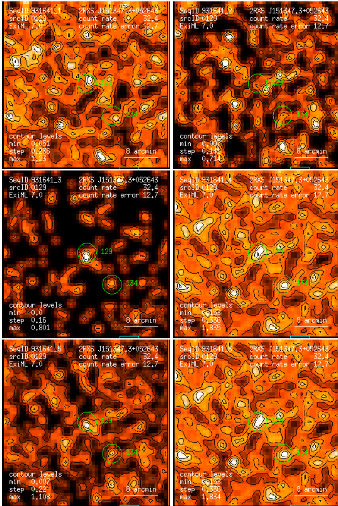
Figure 129: RASS 931641: detection 0129: band rate images, Gaussian filter: (1) PSPC channels 11 – 41, (2) 52 – 90, (3) 91 – 201, (4) 11 – 235, (5) 52 – 201, (6) 11 – 201. Broad band rates in counts/ks. Band rate contour levels in counts/ks/arcmin 2 .
