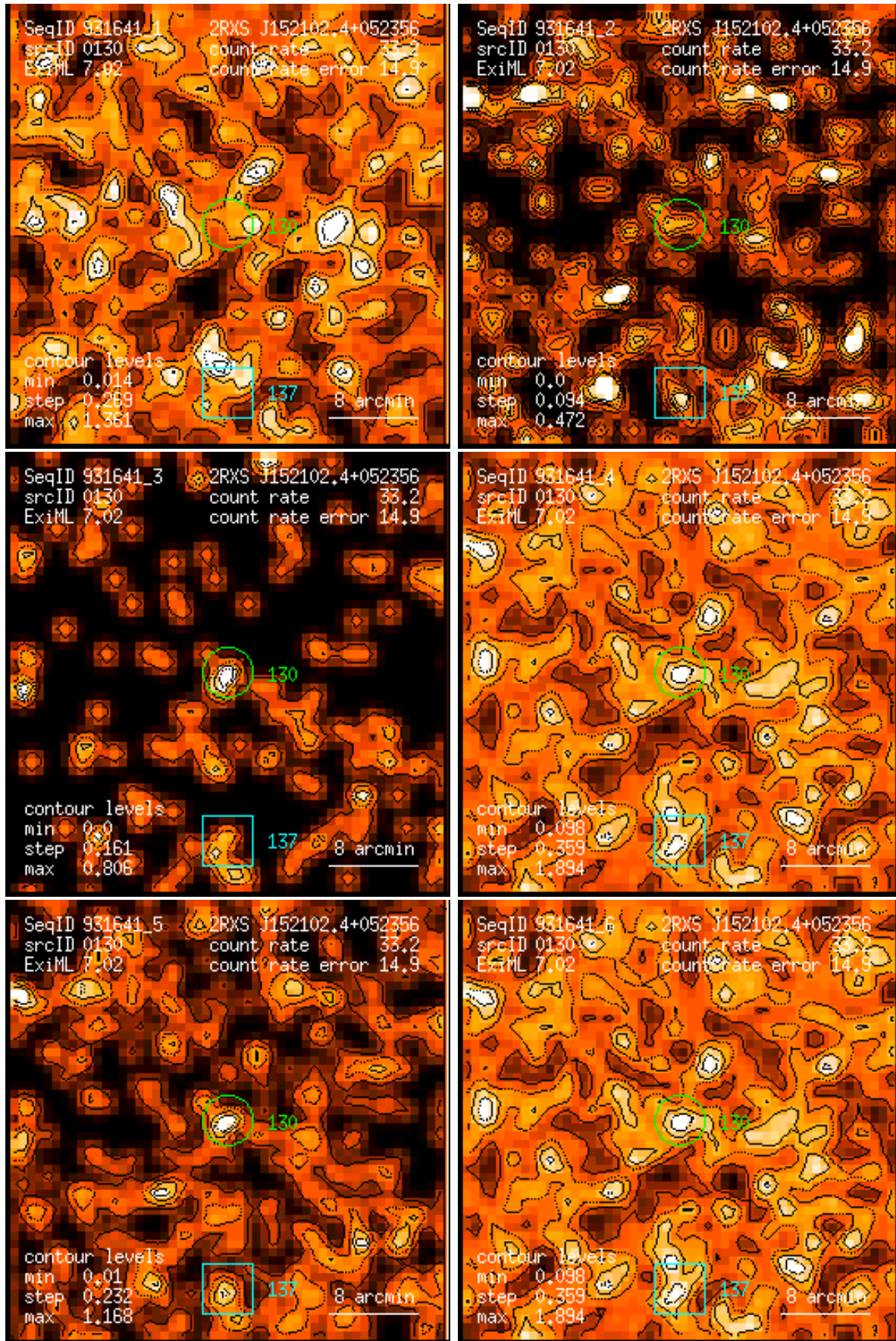
Figure 130: RASS 931641: detection 0130: band rate images, Gaussian filter: (1) PSPC channels 11 – 41, (2) 52 – 90, (3) 91 – 201, (4) 11 – 235, (5) 52 – 201, (6) 11 – 201. Broad band rates in counts/ks. Band rate contour levels in counts/ks/arcmin 2 .
