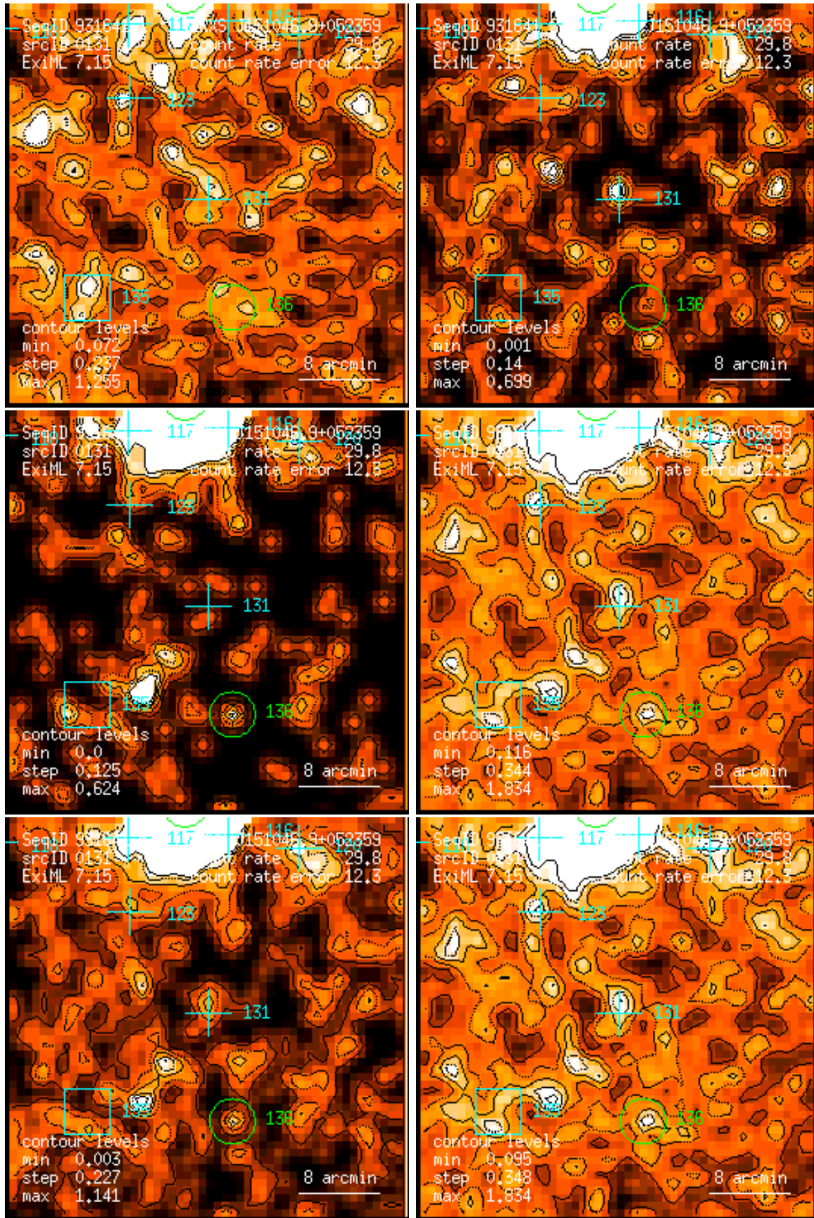
Figure 131: RASS 931641: detection 0131: band rate images, Gaussian filter: (1) PSPC channels 11 – 41, (2) 52 – 90, (3) 91 – 201, (4) 11 – 235, (5) 52 – 201, (6) 11 – 201. Broad band rates in counts/ks. Band rate contour levels in counts/ks/arcmin 2 .
