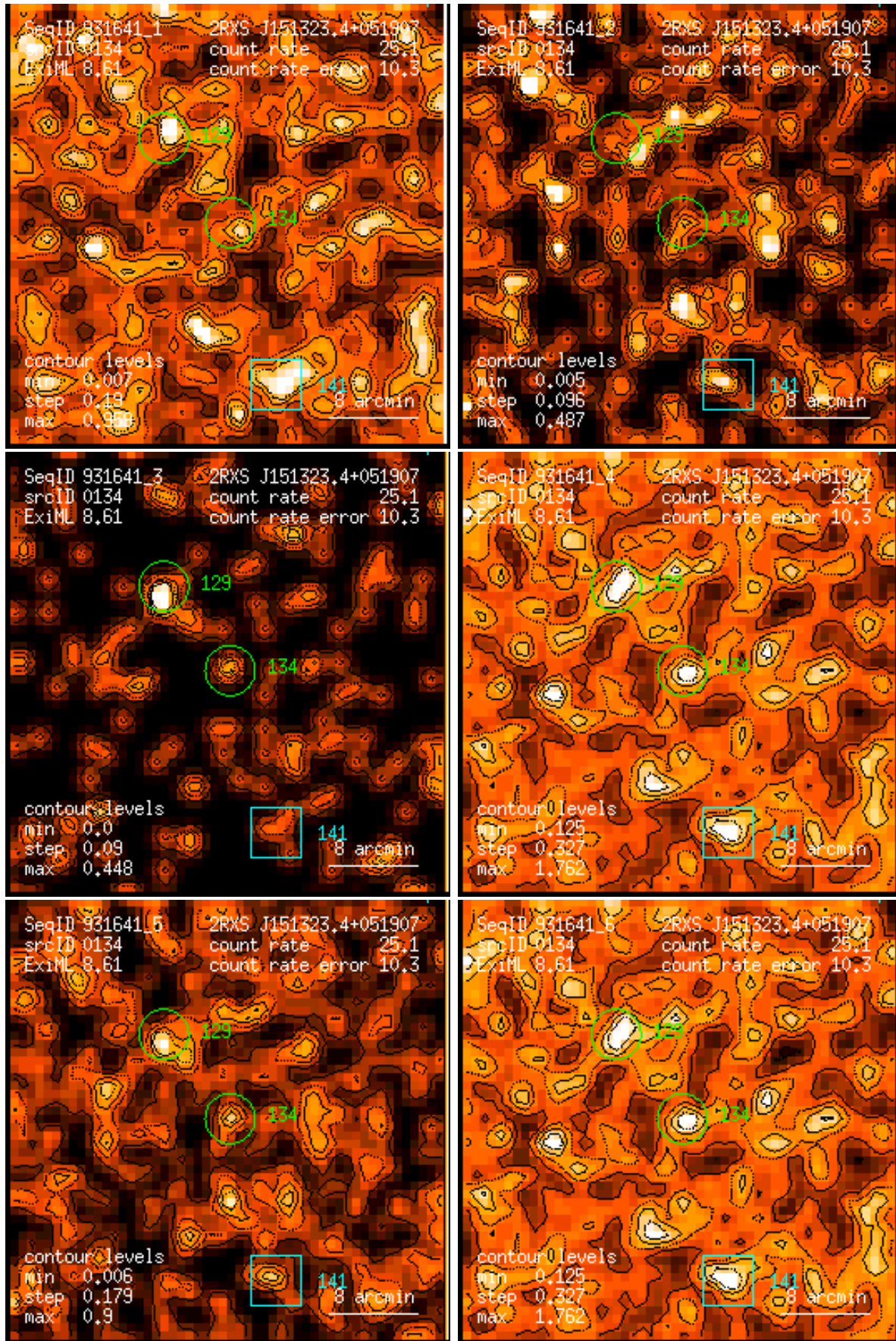
Figure 134: RASS 931641: detection 0134: band rate images, Gaussian filter: (1) PSPC channels 11 – 41, (2) 52 – 90, (3) 91 – 201, (4) 11 – 235, (5) 52 – 201, (6) 11 – 201. Broad band rates in counts/ks. Band rate contour levels in counts/ks/arcmin 2 .
