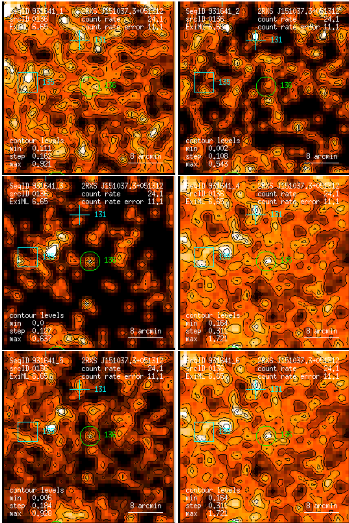
Figure 136: RASS 931641: detection 0136: band rate images, Gaussian filter: (1) PSPC channels 11 – 41, (2) 52 – 90, (3) 91 – 201, (4) 11 – 235, (5) 52 – 201, (6) 11 – 201. Broad band rates in counts/ks. Band rate contour levels in counts/ks/arcmin 2 .
