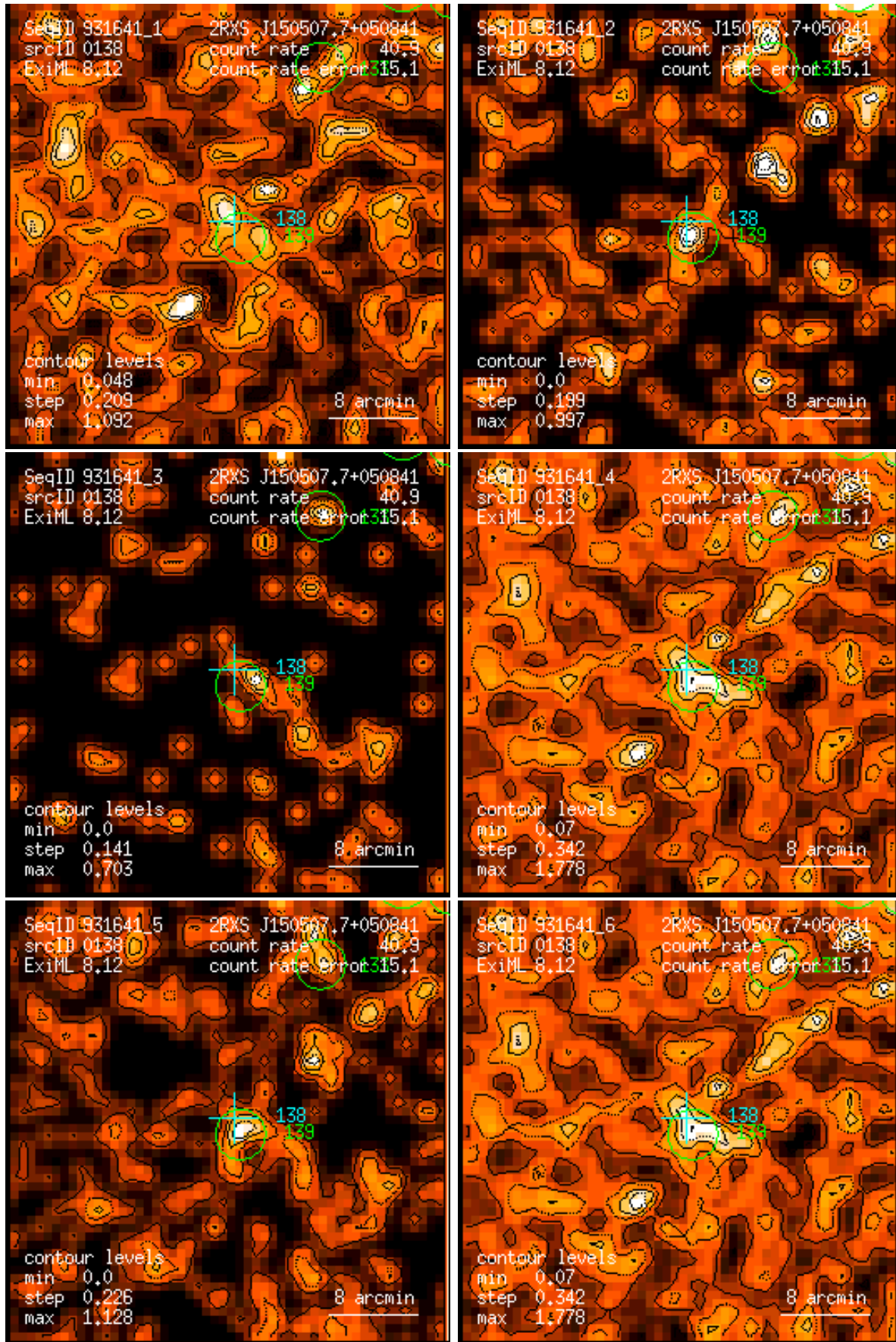
Figure 138: RASS 931641: detection 0138: band rate images, Gaussian filter: (1) PSPC channels 11 – 41, (2) 52 – 90, (3) 91 – 201, (4) 11 – 235, (5) 52 – 201, (6) 11 – 201. Broad band rates in counts/ks. Band rate contour levels in counts/ks/arcmin 2 .
