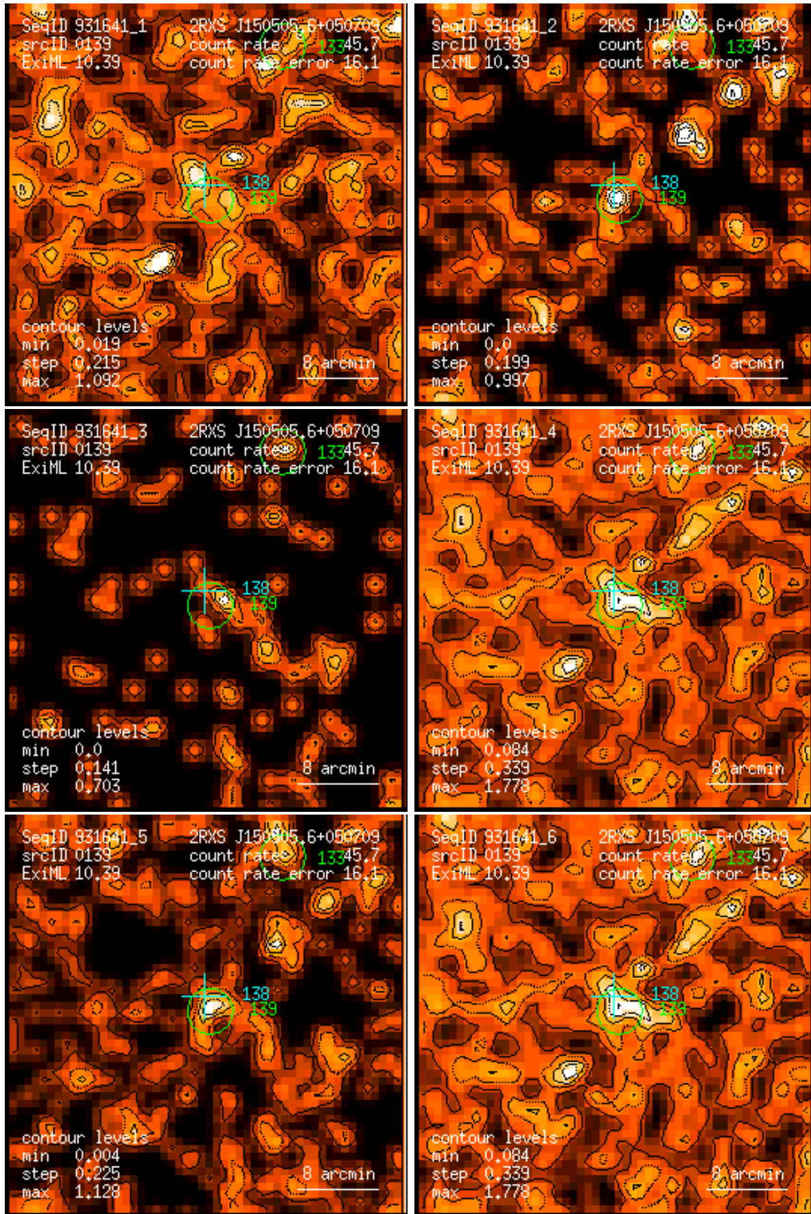
Figure 139: RASS 931641: detection 0139: band rate images, Gaussian filter: (1) PSPC channels 11 – 41, (2) 52 – 90, (3) 91 – 201, (4) 11 – 235, (5) 52 – 201, (6) 11 – 201. Broad band rates in counts/ks. Band rate contour levels in counts/ks/arcmin 2 .
