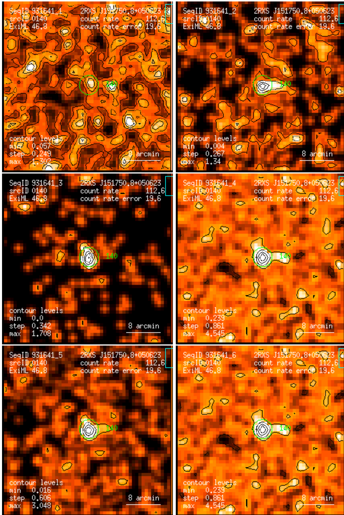
Figure 140: RASS 931641: detection 0140: band rate images, Gaussian filter: (1) PSPC channels 11 – 41, (2) 52 – 90, (3) 91 – 201, (4) 11 – 235, (5) 52 – 201, (6) 11 – 201. Broad band rates in counts/ks. Band rate contour levels in counts/ks/arcmin 2 .
