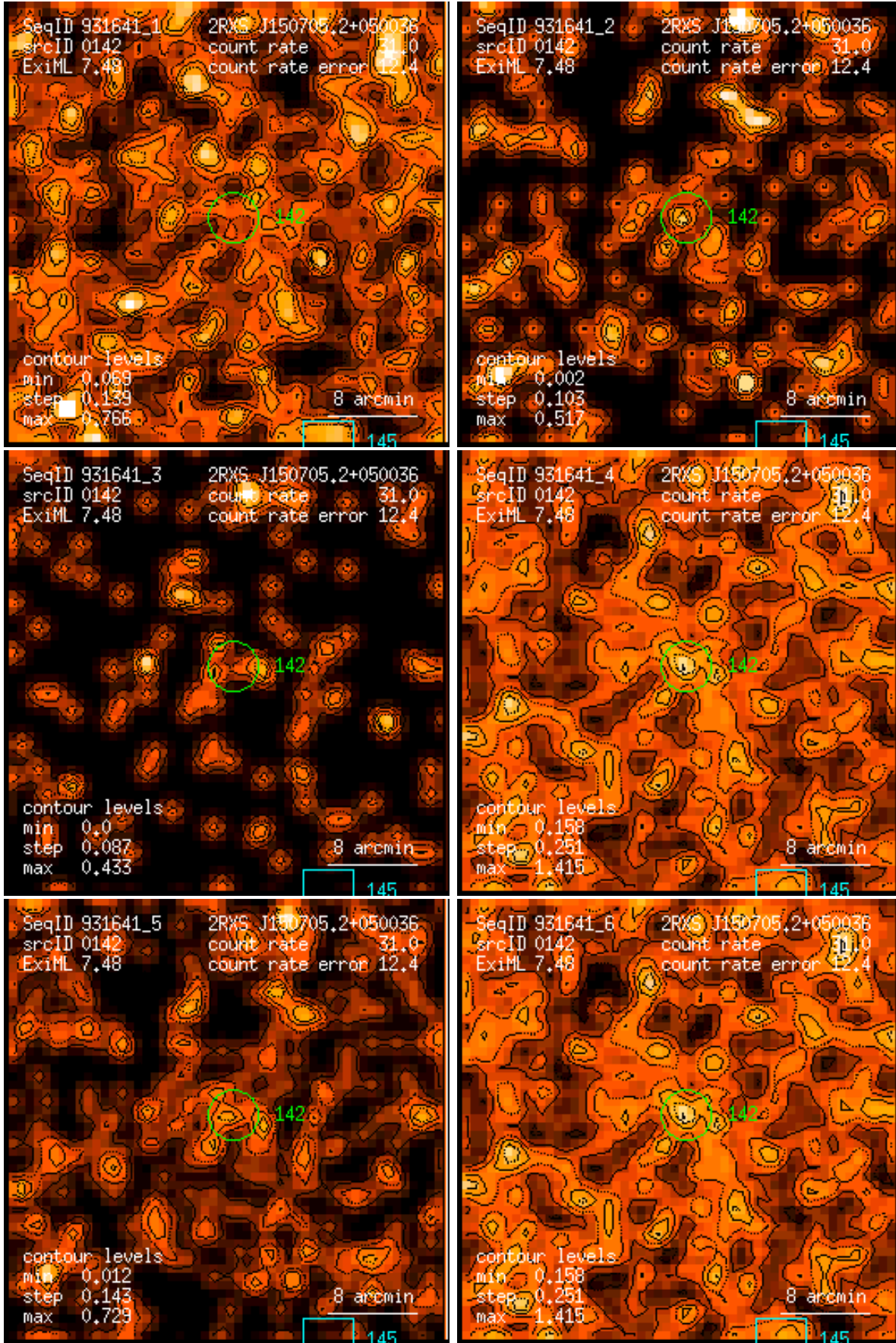
Figure 142: RASS 931641: detection 0142: band rate images, Gaussian filter: (1) PSPC channels 11 – 41, (2) 52 – 90, (3) 91 – 201, (4) 11 – 235, (5) 52 – 201, (6) 11 – 201. Broad band rates in counts/ks. Band rate contour levels in counts/ks/arcmin 2 .
