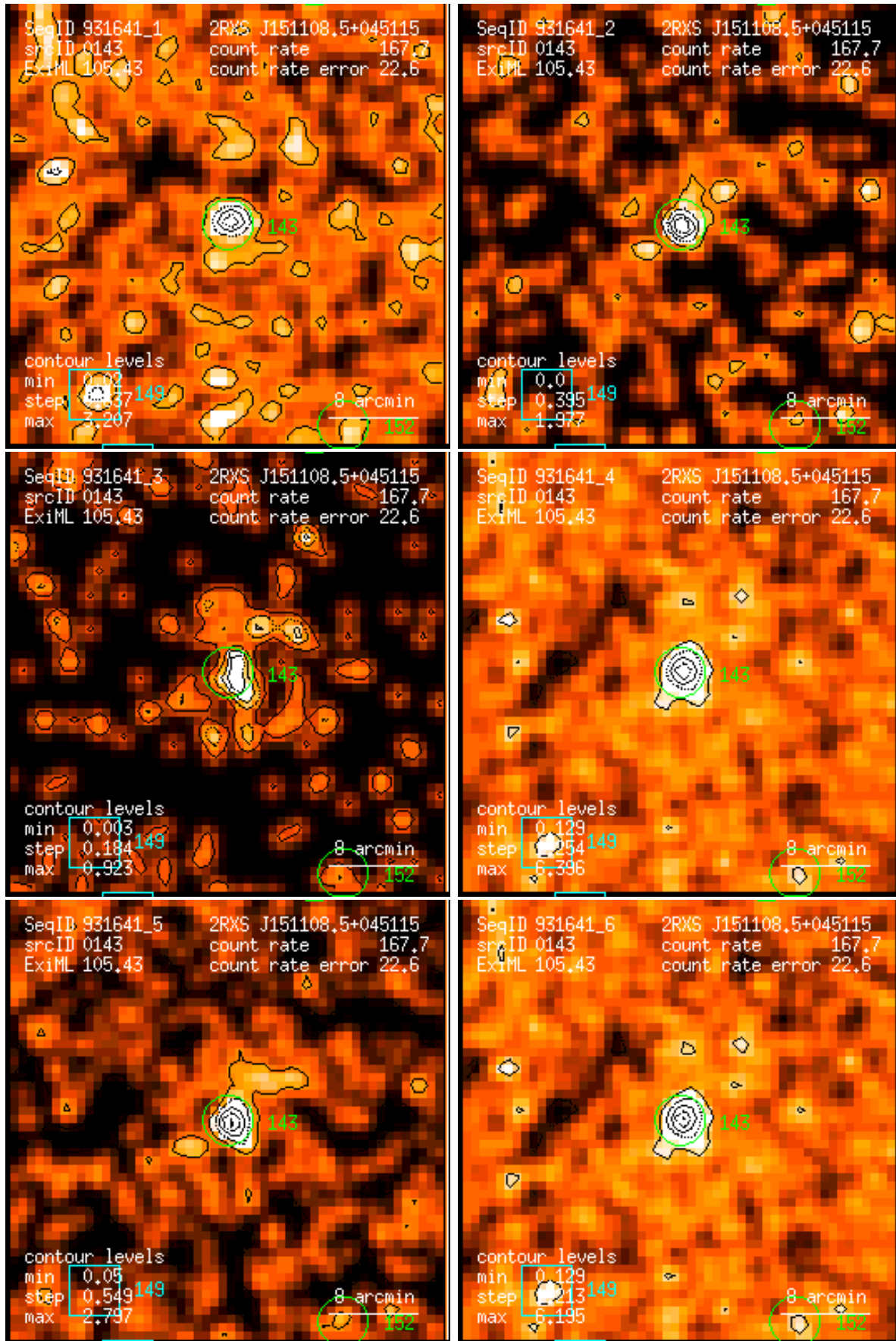
Figure 143: RASS 931641: detection 0143: band rate images, Gaussian filter: (1) PSPC channels 11 – 41, (2) 52 – 90, (3) 91 – 201, (4) 11 – 235, (5) 52 – 201, (6) 11 – 201. Broad band rates in counts/ks. Band rate contour levels in counts/ks/arcmin 2 .
