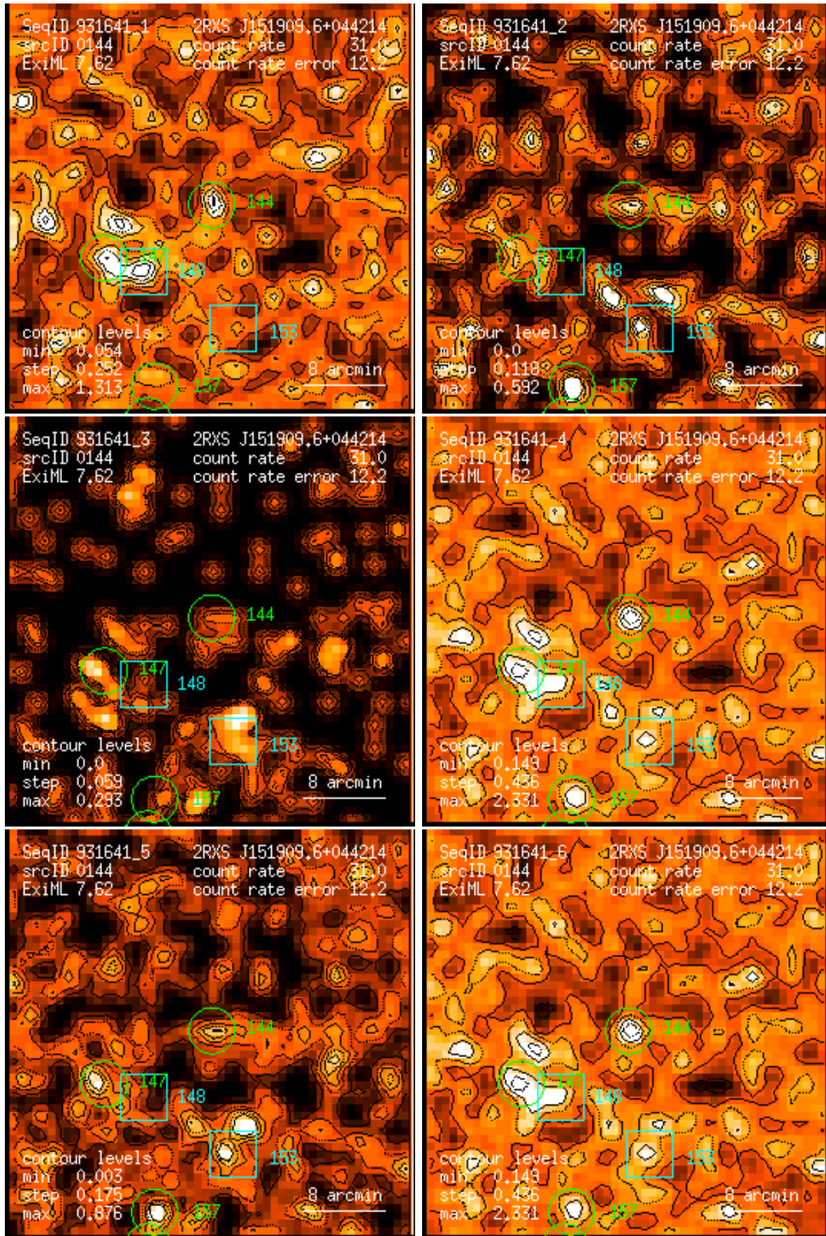
Figure 144: RASS 931641: detection 0144: band rate images, Gaussian filter: (1) PSPC channels 11 – 41, (2) 52 – 90, (3) 91 – 201, (4) 11 – 235, (5) 52 – 201, (6) 11 – 201. Broad band rates in counts/ks. Band rate contour levels in counts/ks/arcmin 2 .
