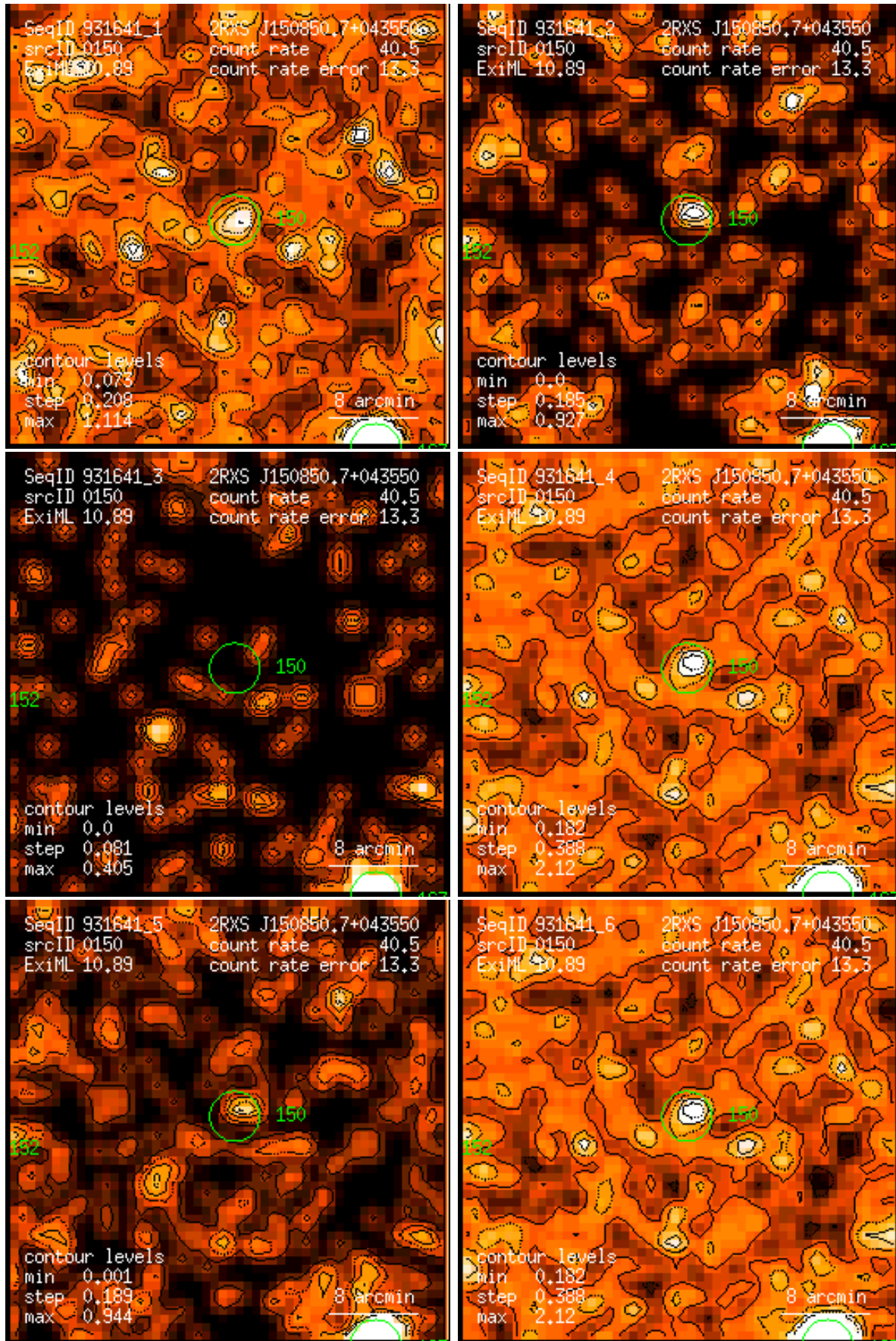
Figure 150: RASS 931641: detection 0150: band rate images, Gaussian filter: (1) PSPC channels 11 – 41, (2) 52 – 90, (3) 91 – 201, (4) 11 – 235, (5) 52 – 201, (6) 11 – 201. Broad band rates in counts/ks. Band rate contour levels in counts/ks/arcmin 2 .
