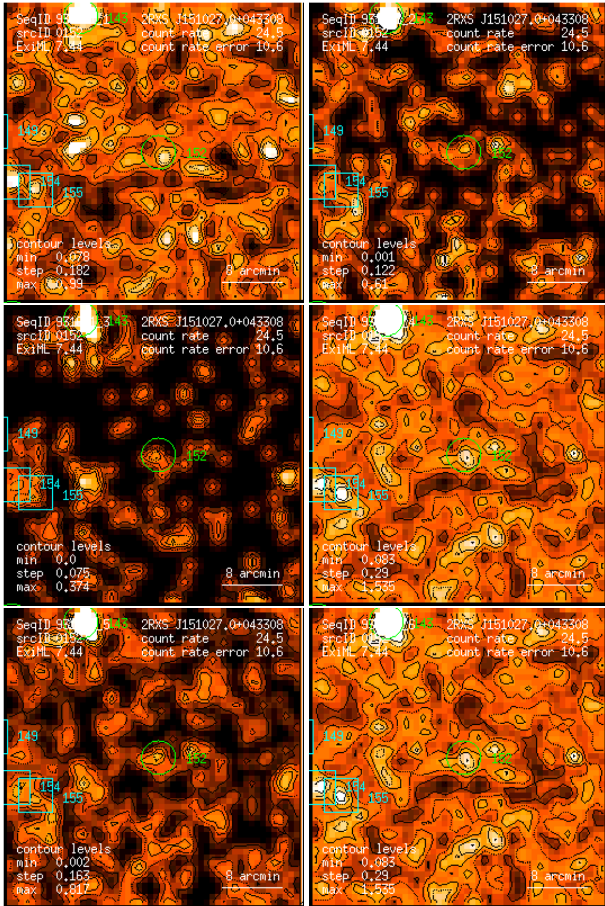
Figure 152: RASS 931641: detection 0152: band rate images, Gaussian filter: (1) PSPC channels 11 – 41, (2) 52 – 90, (3) 91 – 201, (4) 11 – 235, (5) 52 – 201, (6) 11 – 201. Broad band rates in counts/ks. Band rate contour levels in counts/ks/arcmin 2 .
