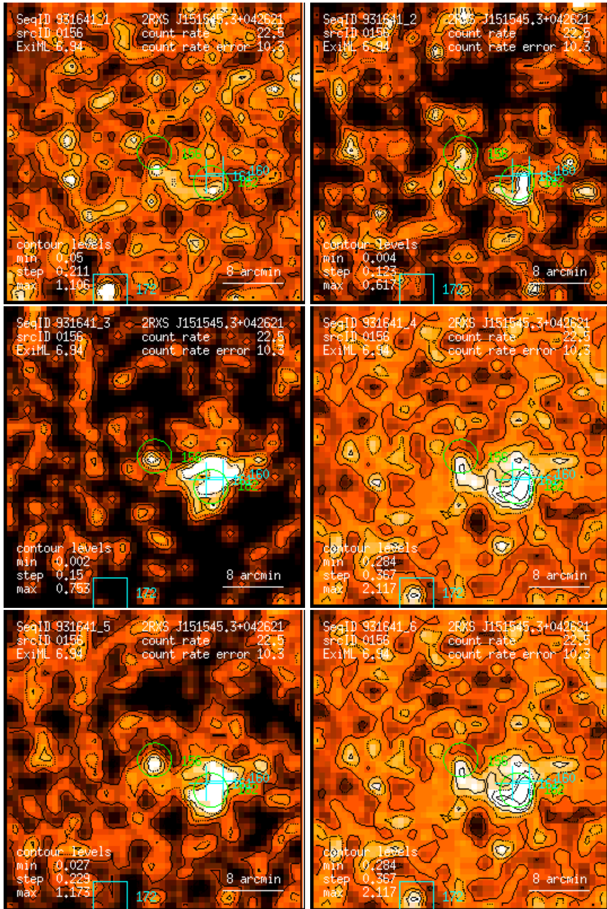
Figure 156: RASS 931641: detection 0156: band rate images, Gaussian filter: (1) PSPC channels 11 – 41, (2) 52 – 90, (3) 91 – 201, (4) 11 – 235, (5) 52 – 201, (6) 11 – 201. Broad band rates in counts/ks. Band rate contour levels in counts/ks/arcmin 2 .
