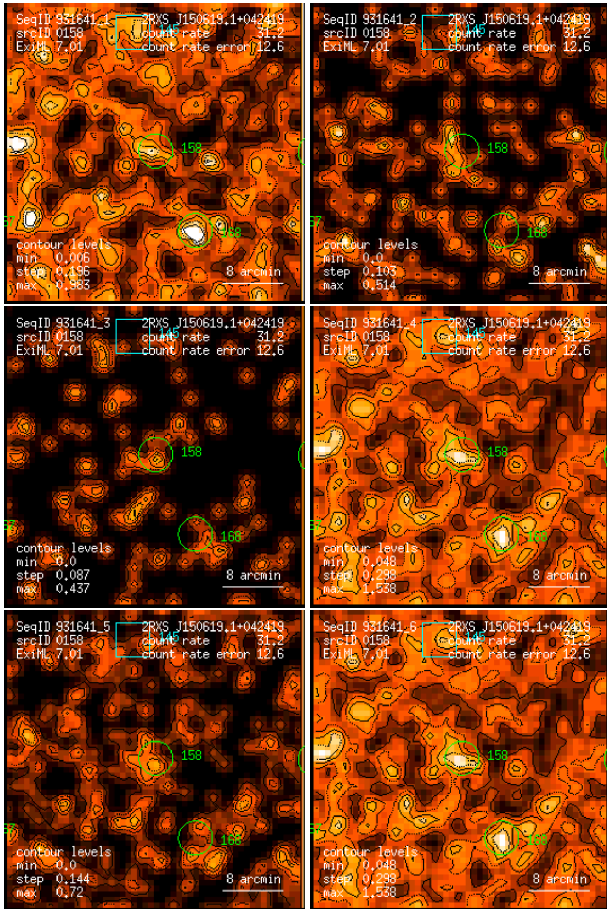
Figure 158: RASS 931641: detection 0158: band rate images, Gaussian filter: (1) PSPC channels 11 – 41, (2) 52 – 90, (3) 91 – 201, (4) 11 – 235, (5) 52 – 201, (6) 11 – 201. Broad band rates in counts/ks. Band rate contour levels in counts/ks/arcmin 2 .
