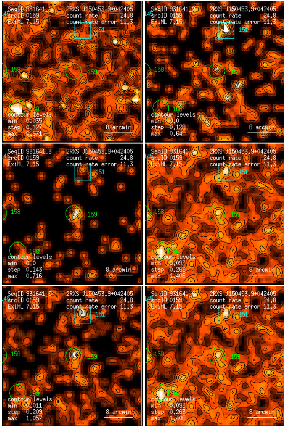
Figure 159: RASS 931641: detection 0159: band rate images, Gaussian filter: (1) PSPC channels 11 – 41, (2) 52 – 90, (3) 91 – 201, (4) 11 – 235, (5) 52 – 201, (6) 11 – 201. Broad band rates in counts/ks. Band rate contour levels in counts/ks/arcmin 2 .
