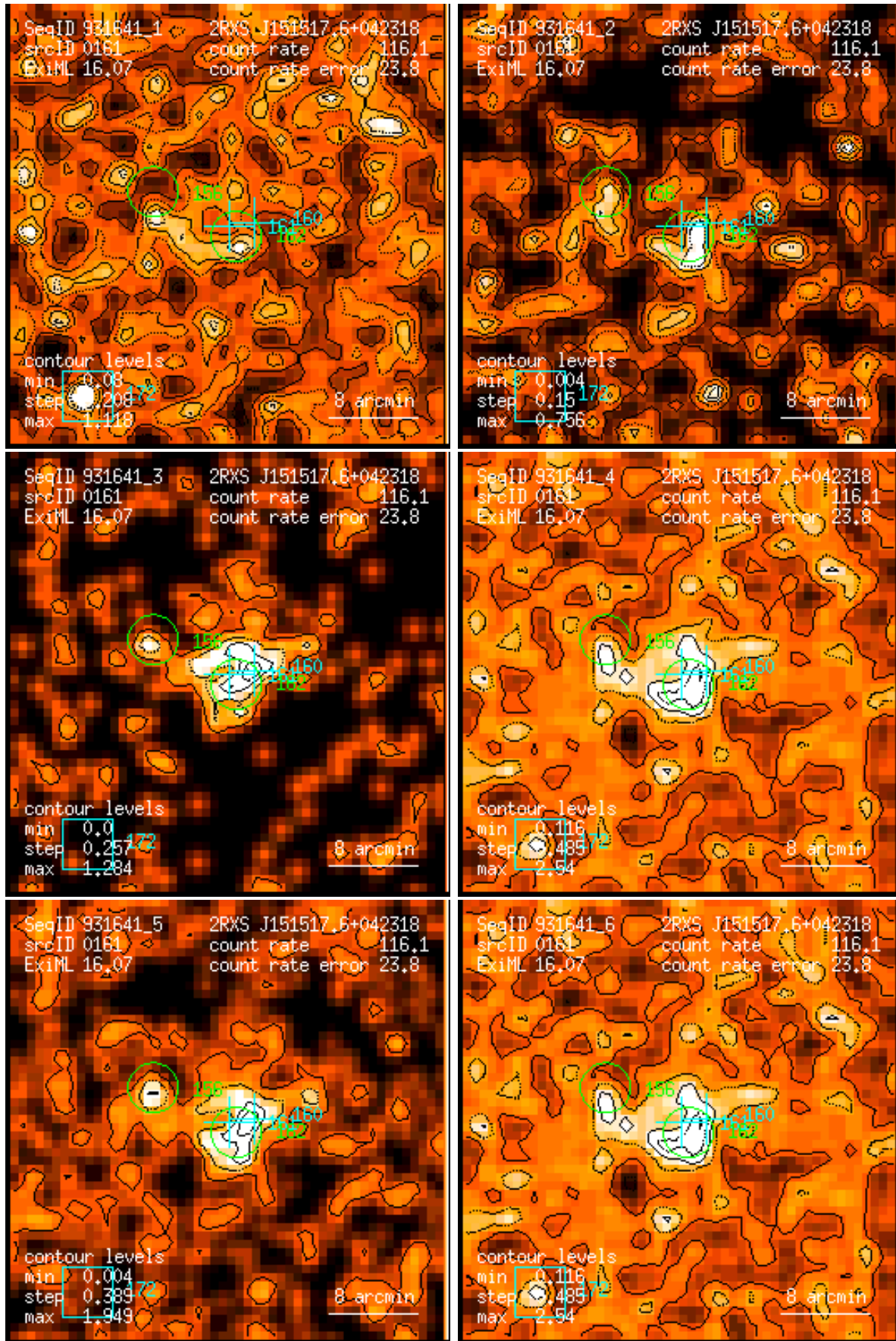
Figure 161: RASS 931641: detection 0161: band rate images, Gaussian filter: (1) PSPC channels 11 – 41, (2) 52 – 90, (3) 91 – 201, (4) 11 – 235, (5) 52 – 201, (6) 11 – 201. Broad band rates in counts/ks. Band rate contour levels in counts/ks/arcmin 2 .
