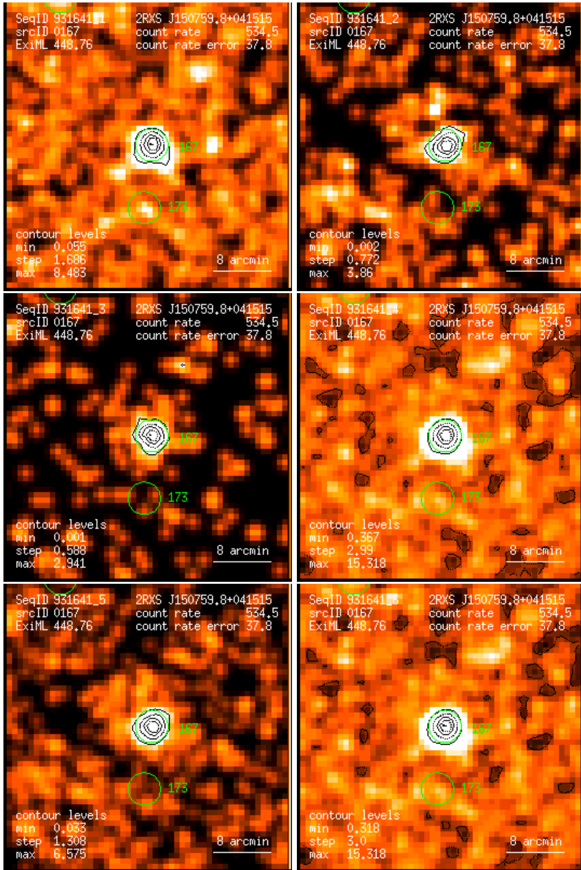
Figure 167: RASS 931641: detection 0167: band rate images, Gaussian filter: (1) PSPC channels 11 – 41, (2) 52 – 90, (3) 91 – 201, (4) 11 – 235, (5) 52 – 201, (6) 11 – 201. Broad band rates in counts/ks. Band rate contour levels in counts/ks/arcmin 2 .
