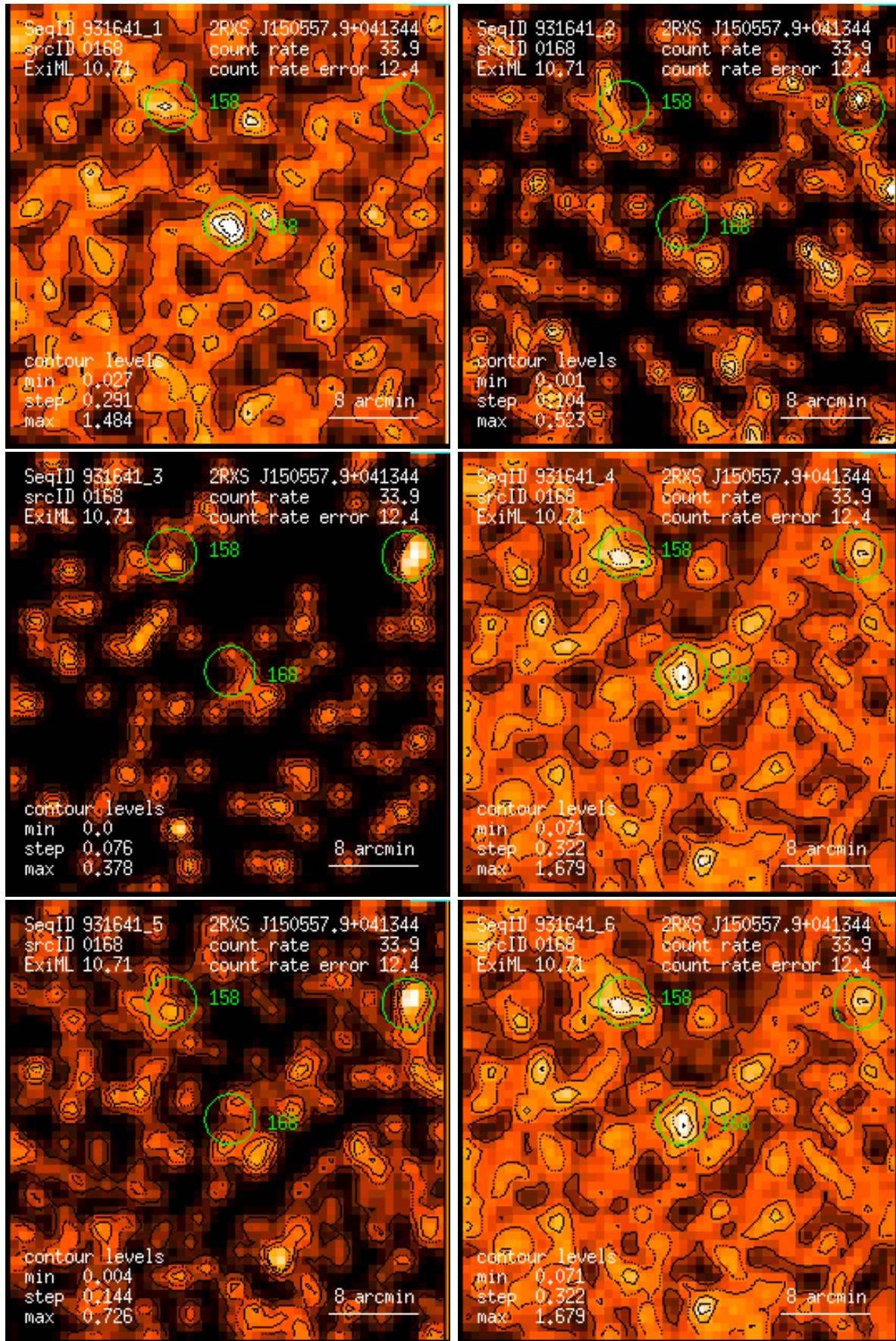
Figure 168: RASS 931641: detection 0168: band rate images, Gaussian filter: (1) PSPC channels 11 – 41, (2) 52 – 90, (3) 91 – 201, (4) 11 – 235, (5) 52 – 201, (6) 11 – 201. Broad band rates in counts/ks. Band rate contour levels in counts/ks/arcmin 2 .
