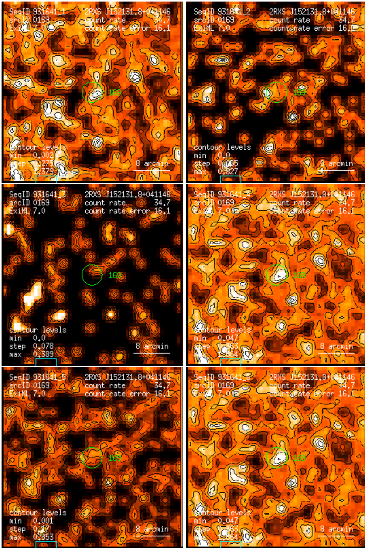
Figure 169: RASS 931641: detection 0169: band rate images, Gaussian filter: (1) PSPC channels 11 – 41, (2) 52 – 90, (3) 91 – 201, (4) 11 – 235, (5) 52 – 201, (6) 11 – 201. Broad band rates in counts/ks. Band rate contour levels in counts/ks/arcmin 2 .
