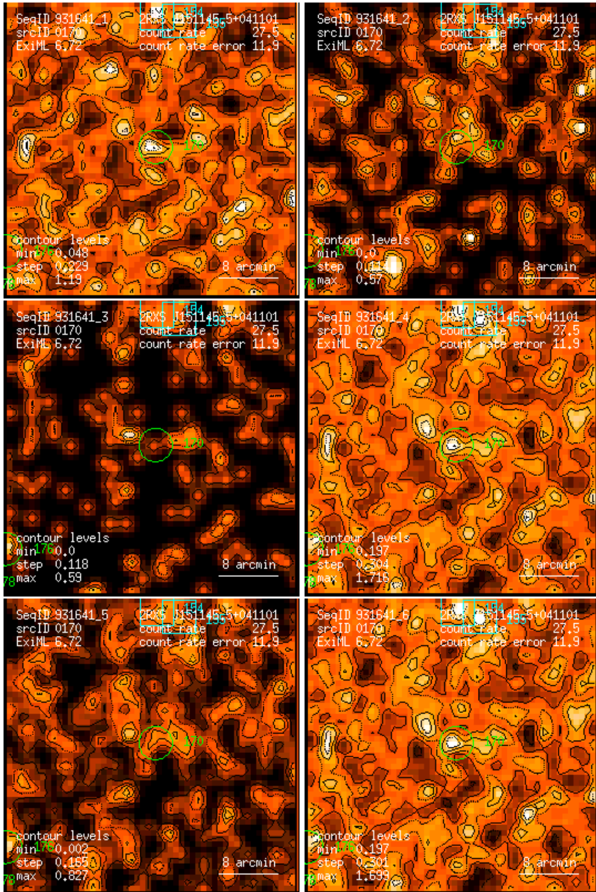
Figure 170: RASS 931641: detection 0170: band rate images, Gaussian filter: (1) PSPC channels 11 – 41, (2) 52 – 90, (3) 91 – 201, (4) 11 – 235, (5) 52 – 201, (6) 11 – 201. Broad band rates in counts/ks. Band rate contour levels in counts/ks/arcmin 2 .
