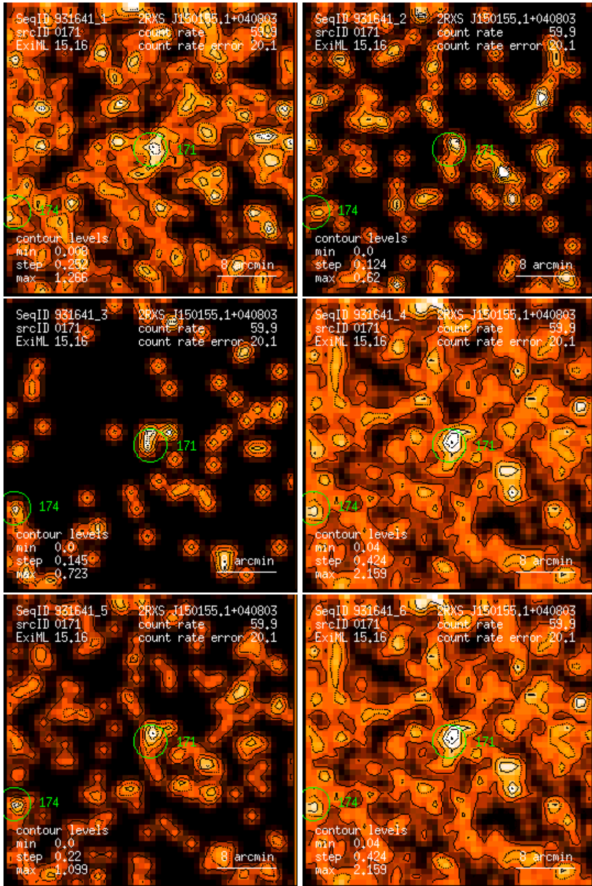
Figure 171: RASS 931641: detection 0171: band rate images, Gaussian filter: (1) PSPC channels 11 – 41, (2) 52 – 90, (3) 91 – 201, (4) 11 – 235, (5) 52 – 201, (6) 11 – 201. Broad band rates in counts/ks. Band rate contour levels in counts/ks/arcmin 2 .
