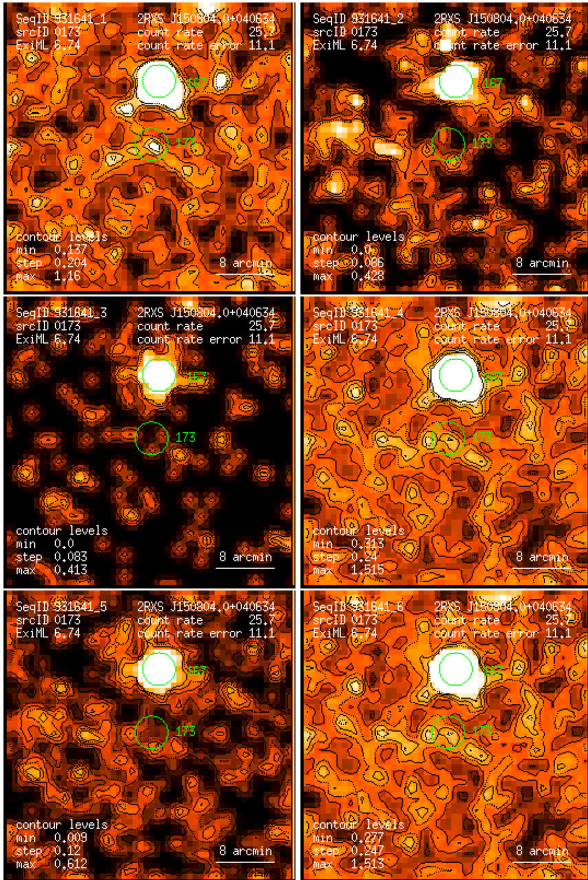
Figure 173: RASS 931641: detection 0173: band rate images, Gaussian filter: (1) PSPC channels 11 – 41, (2) 52 – 90, (3) 91 – 201, (4) 11 – 235, (5) 52 – 201, (6) 11 – 201. Broad band rates in counts/ks. Band rate contour levels in counts/ks/arcmin 2 .
