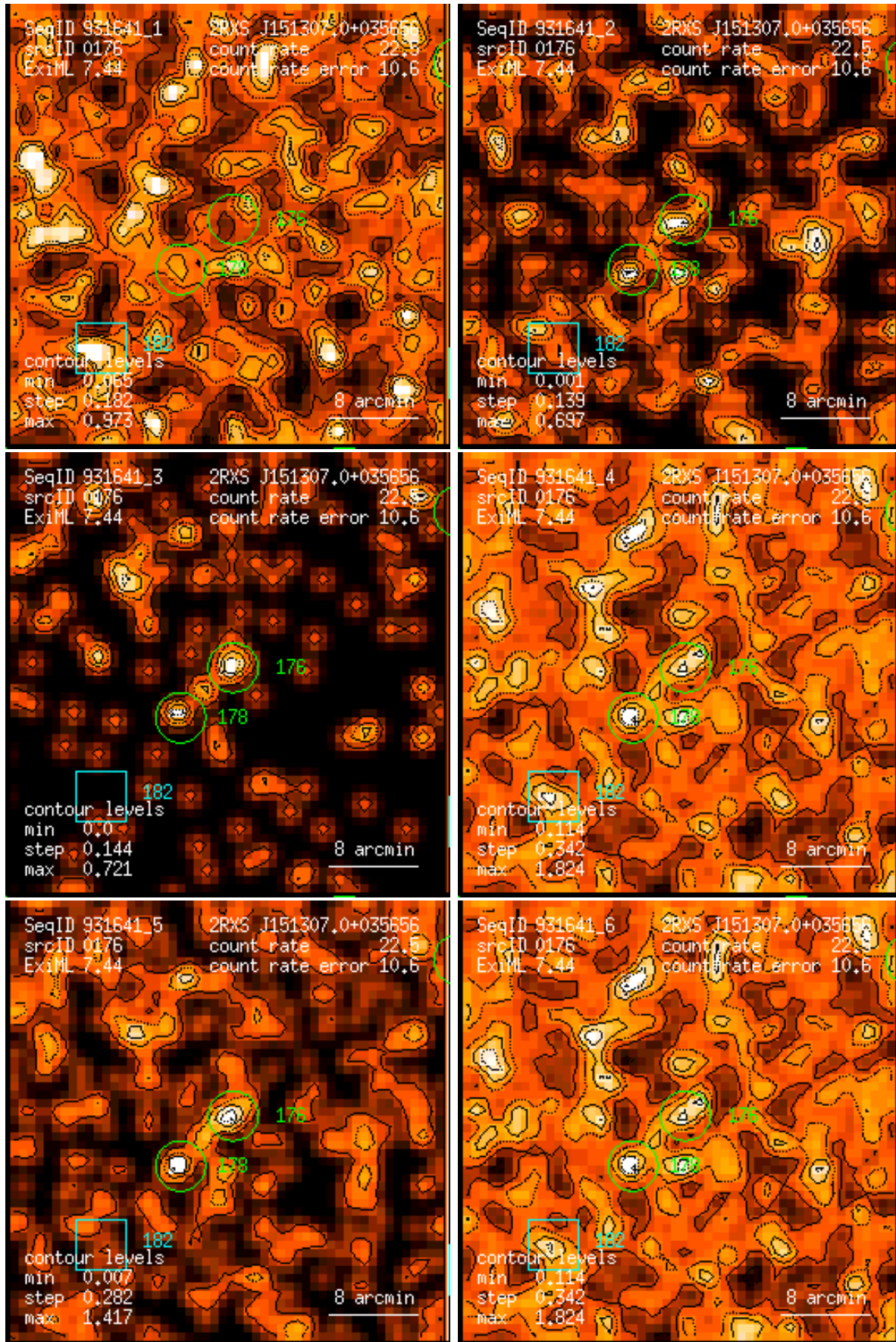
Figure 176: RASS 931641: detection 0176: band rate images, Gaussian filter: (1) PSPC channels 11 – 41, (2) 52 – 90, (3) 91 – 201, (4) 11 – 235, (5) 52 – 201, (6) 11 – 201. Broad band rates in counts/ks. Band rate contour levels in counts/ks/arcmin 2 .
